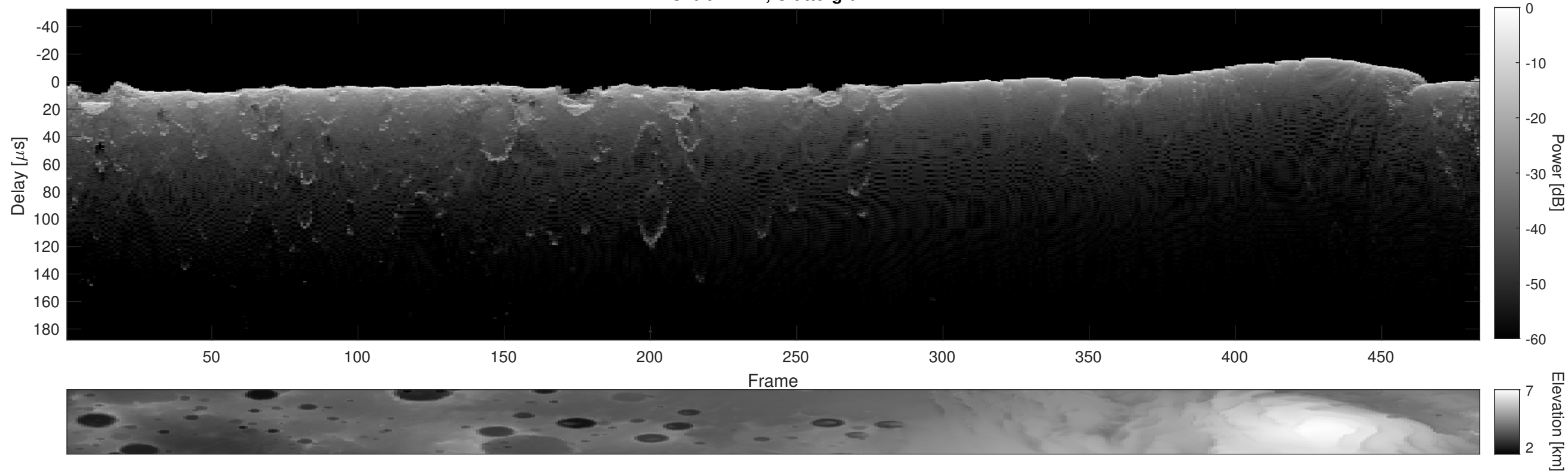
Orbit 21211, Cluttergram
