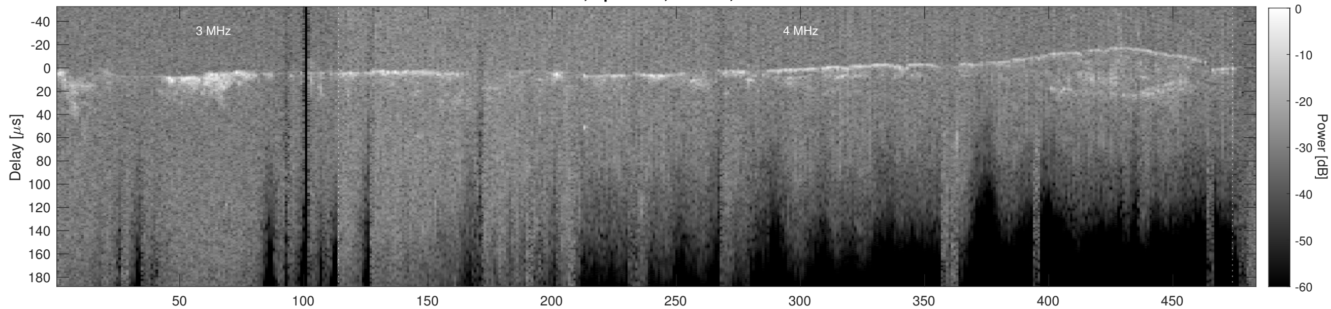
Orbit 21211, Cluttergram
