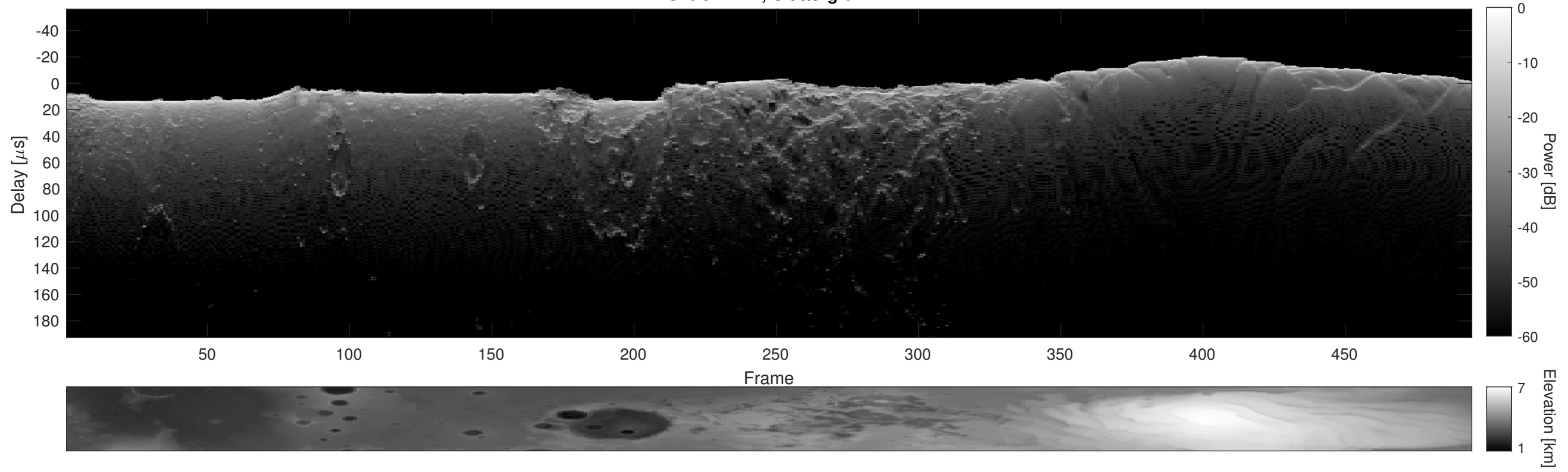
Orbit 21214, Cluttergram
