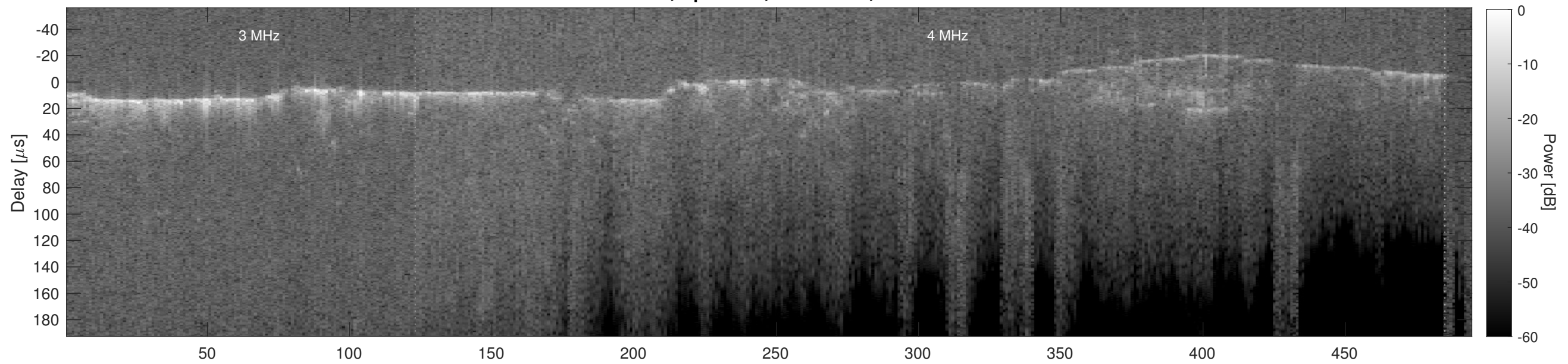
Orbit 21214, Cluttergram
