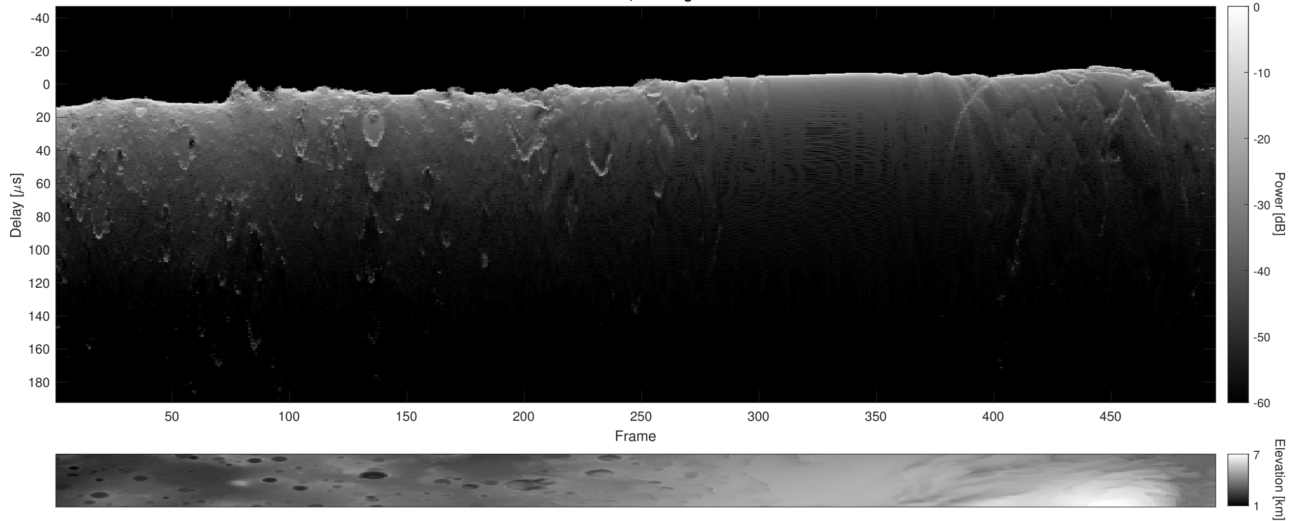
Orbit 21215, Cluttergram
