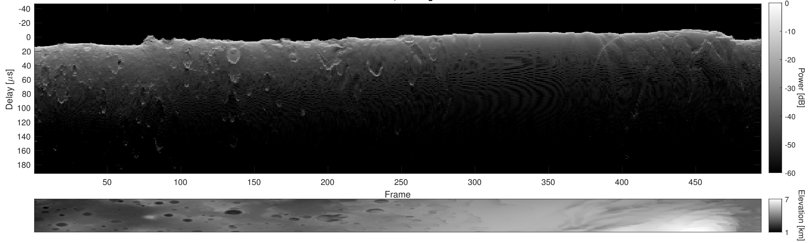
Orbit 21215, Cluttergram
