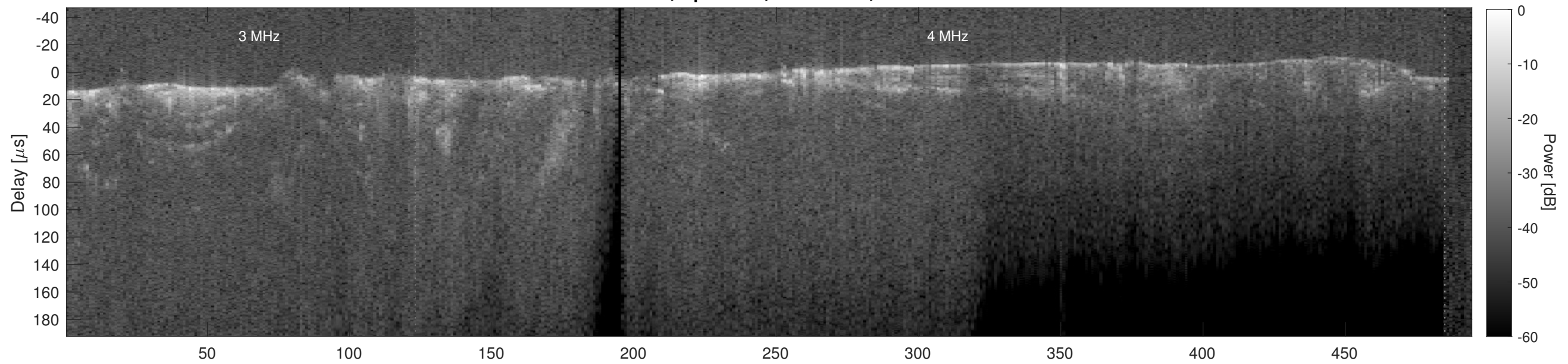
Orbit 21215, Cluttergram
