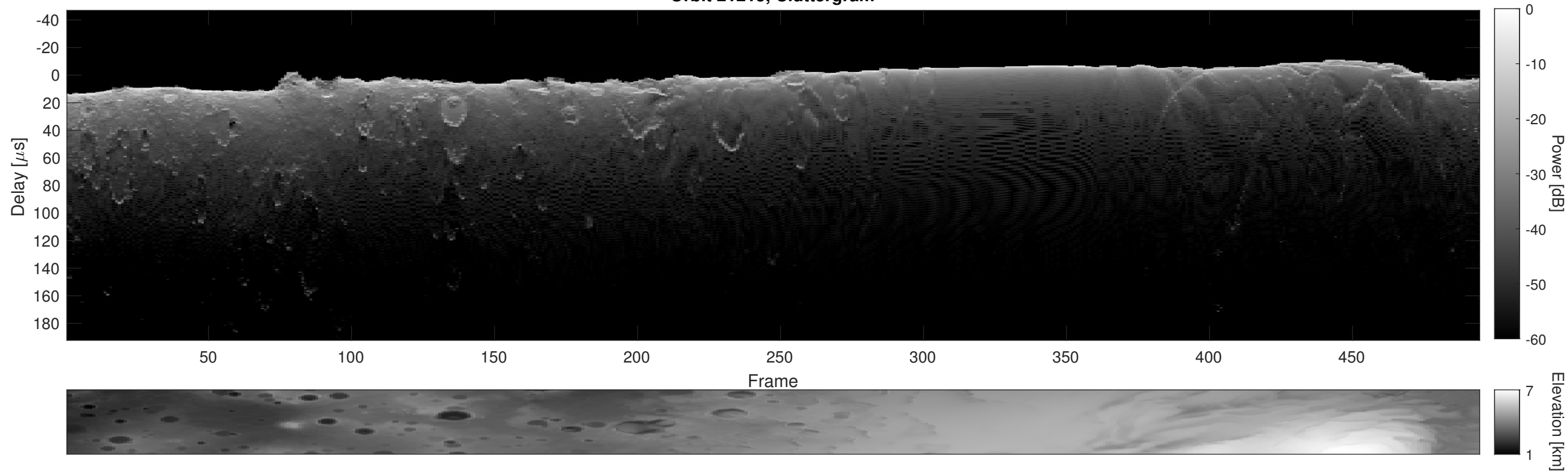
Orbit 21215, Cluttergram
