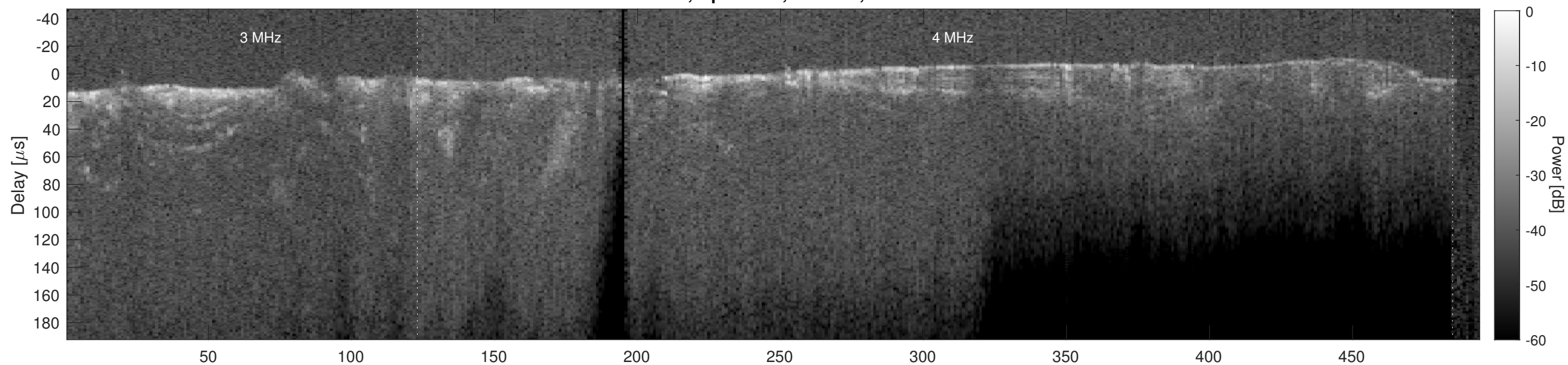
Orbit 21215, Cluttergram
