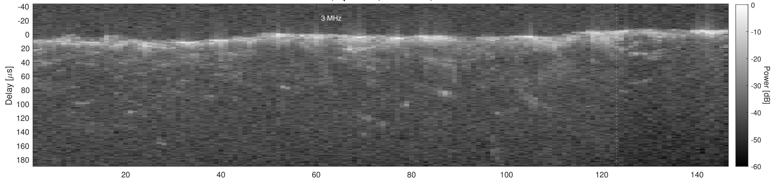
Orbit 21217, Cluttergram
