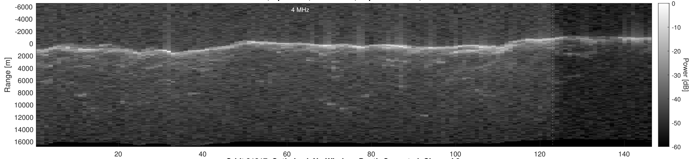
Orbit 21217, Optimized, No Window, Depth-Corrected, Channel 2
