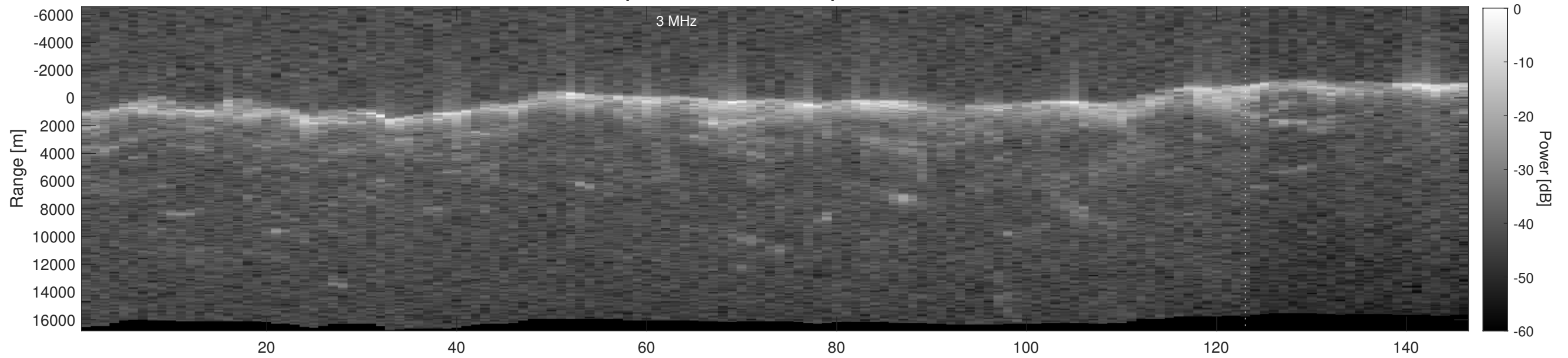
Orbit 21217, Depth-Corrected Cluttergram
