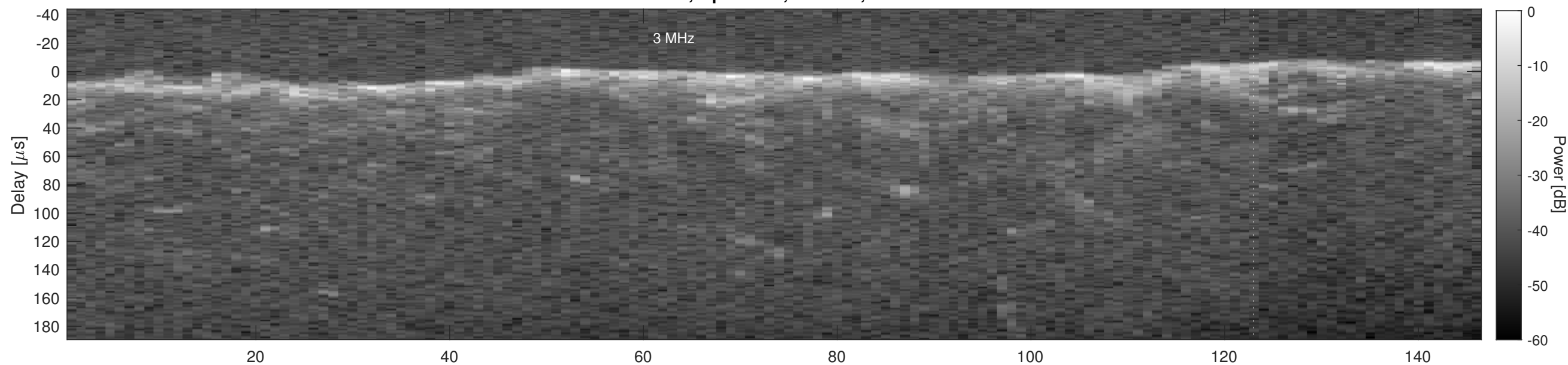
Orbit 21217, Cluttergram
