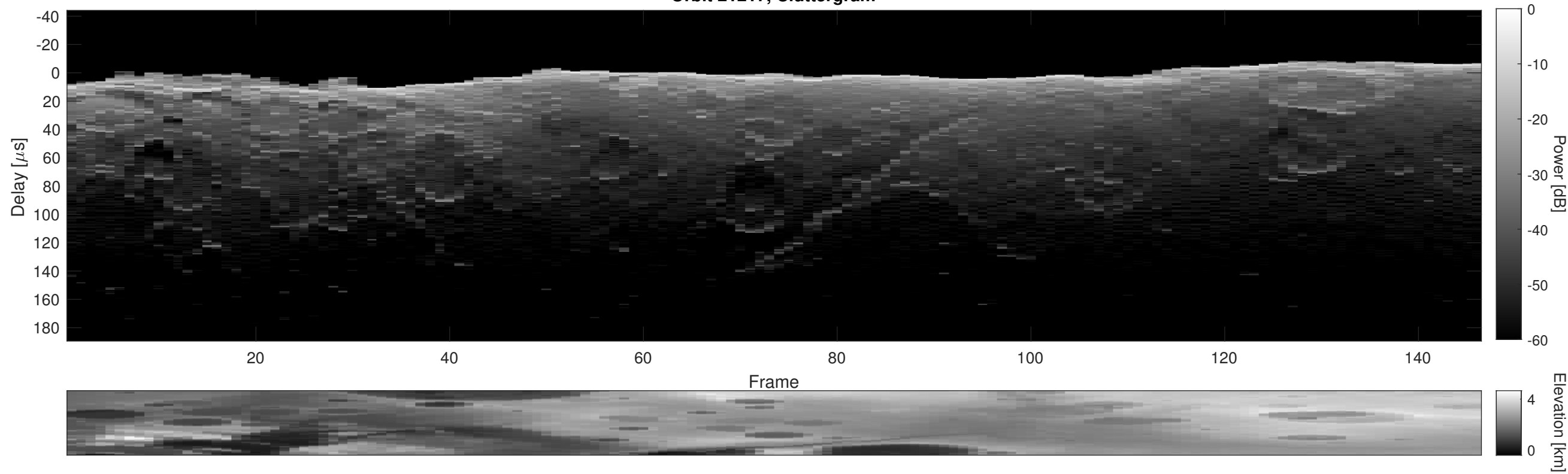
Orbit 21217, Cluttergram
