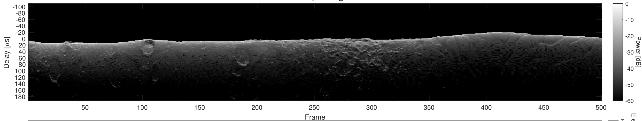
Orbit 21221, Cluttergram
