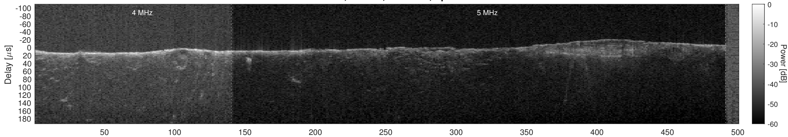
Orbit 21221, Cluttergram
