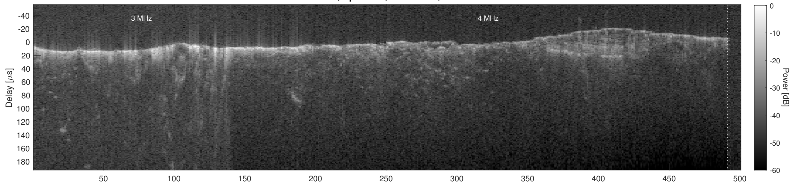
Orbit 21221, Cluttergram
