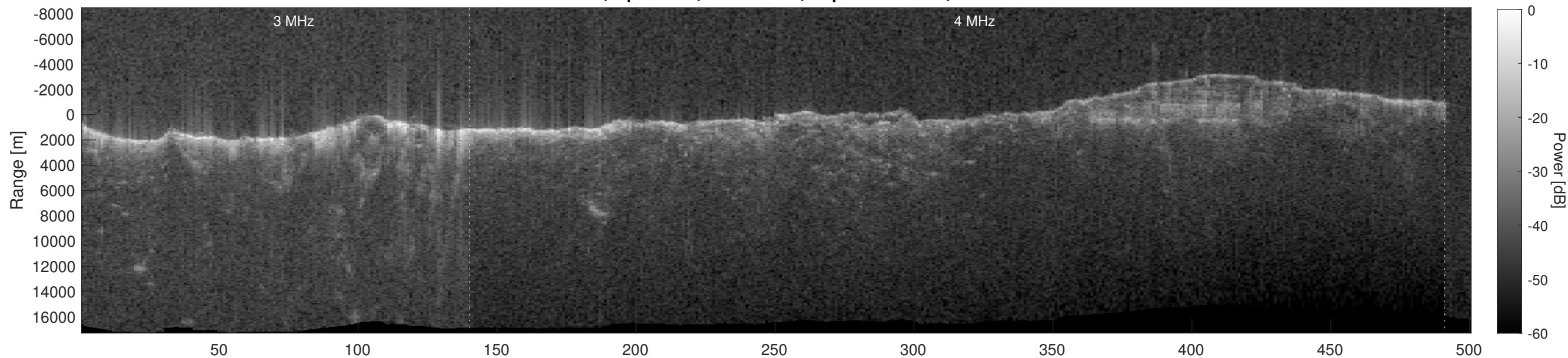
Orbit 21221, Depth-Corrected Cluttergram
