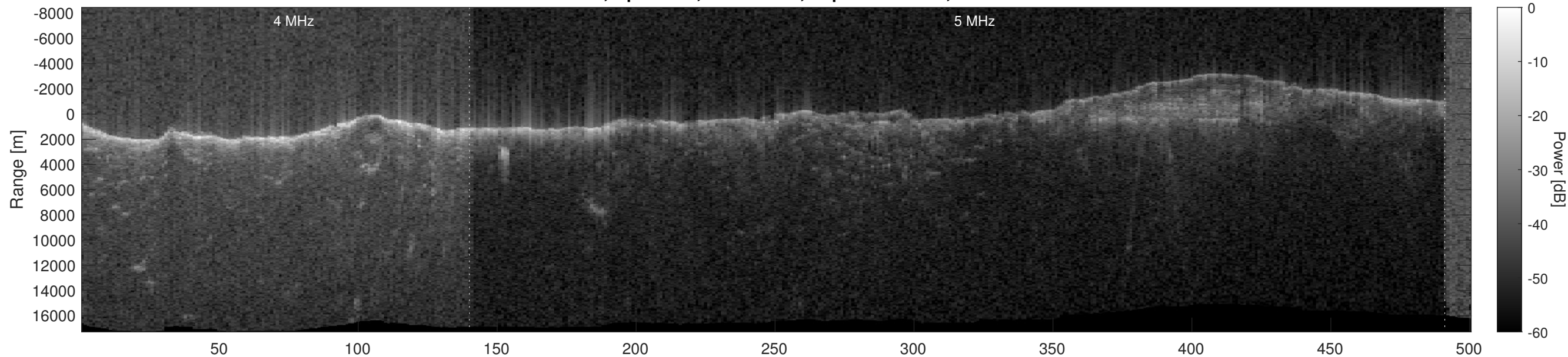
Orbit 21221, Optimized, No Window, Depth-Corrected, Channel 2
