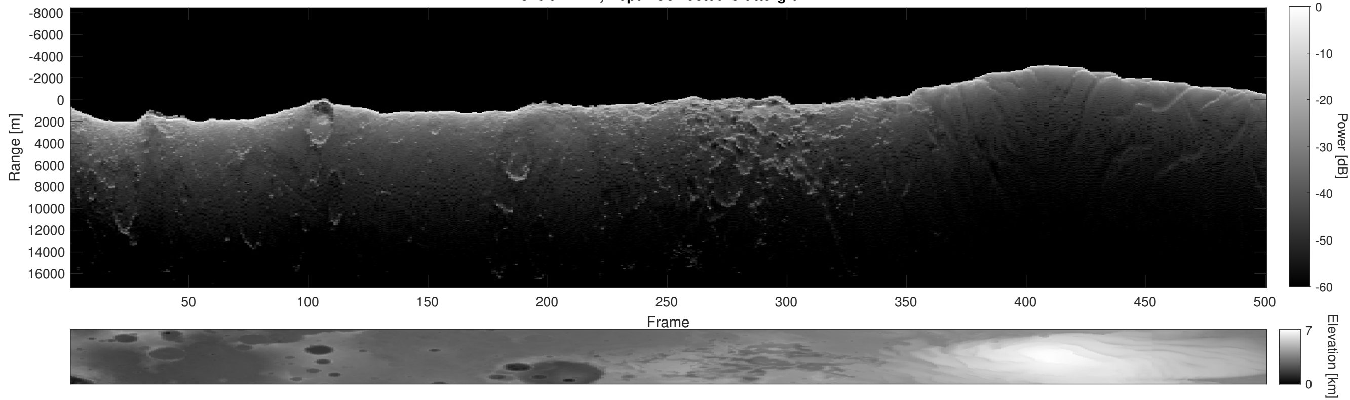
Orbit 21221, Depth-Corrected Cluttergram
