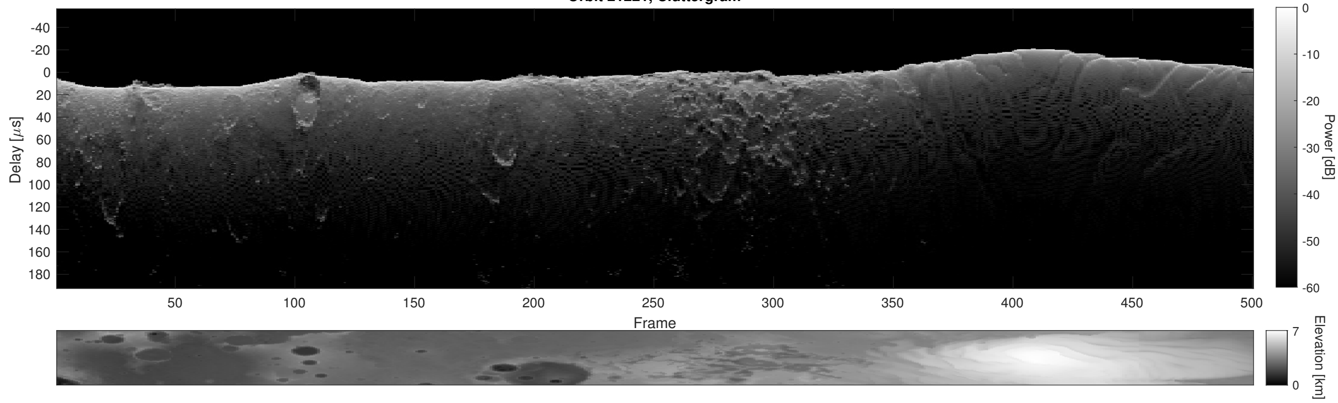
Orbit 21221, Cluttergram
