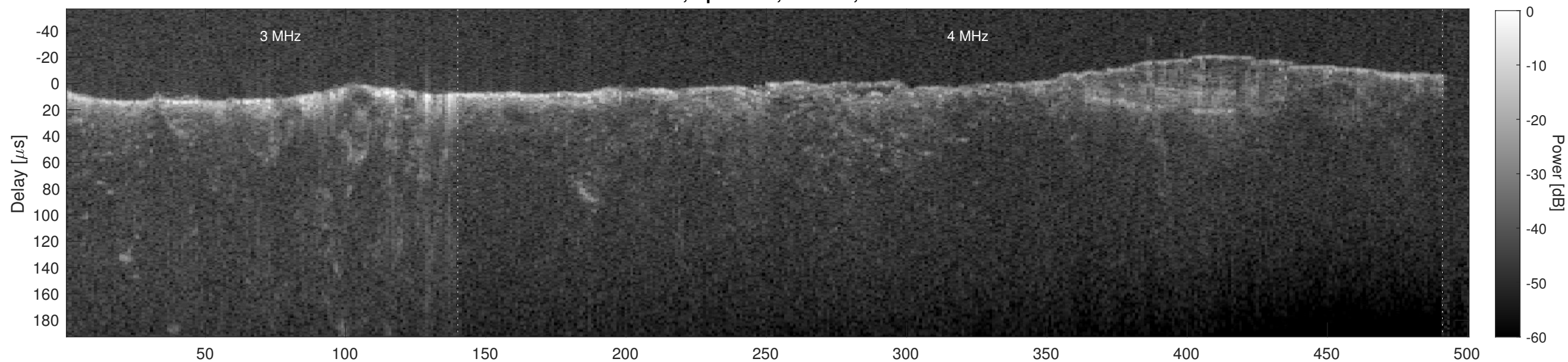
Orbit 21221, Cluttergram
