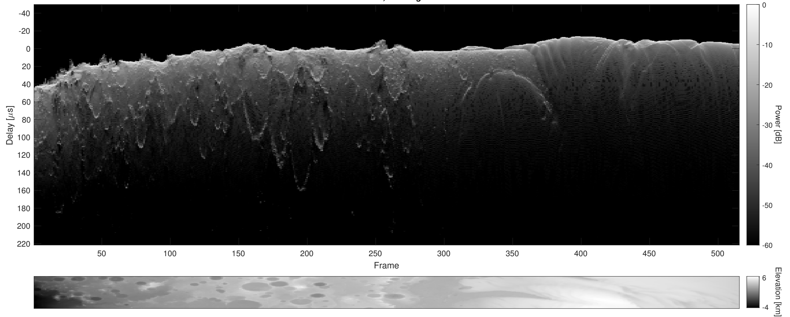
Orbit 21223, Cluttergram
