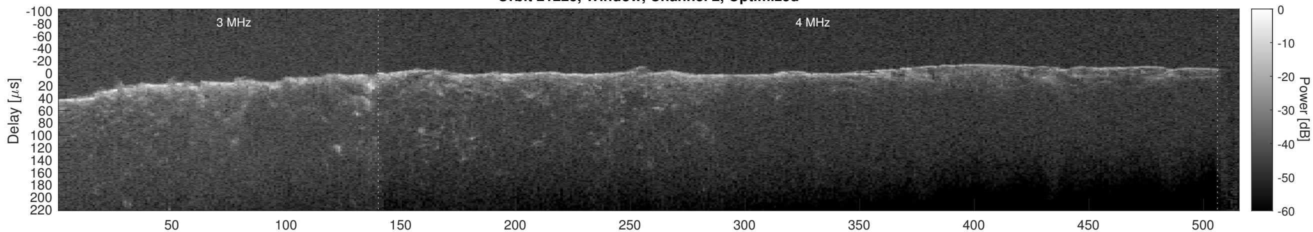
Orbit 21223, Cluttergram
