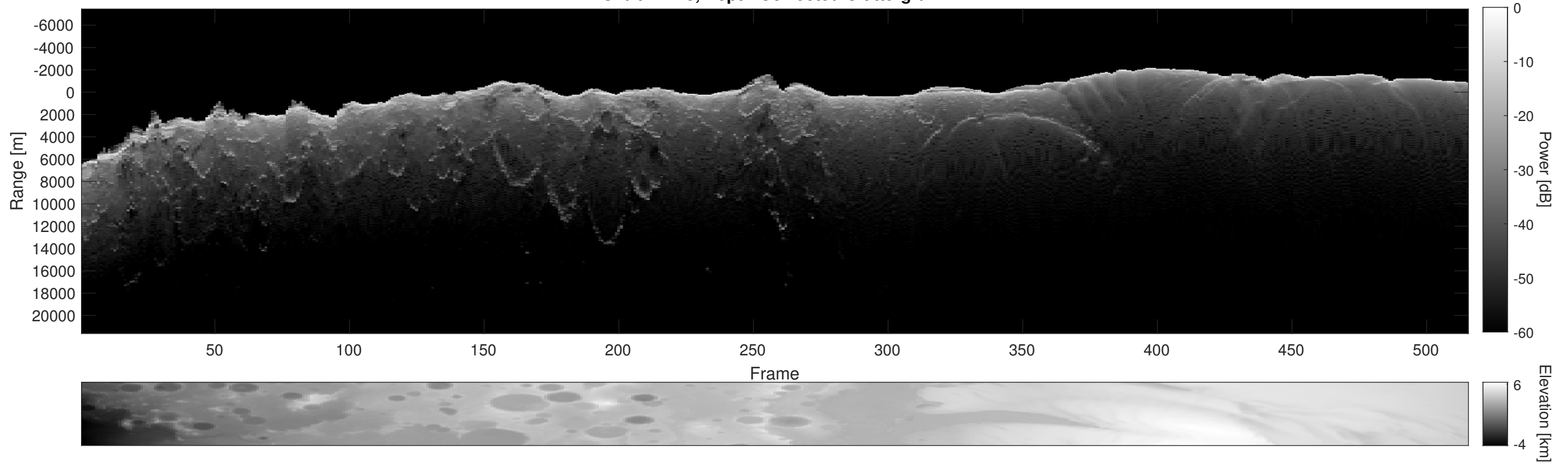
Orbit 21223, Depth-Corrected Cluttergram
