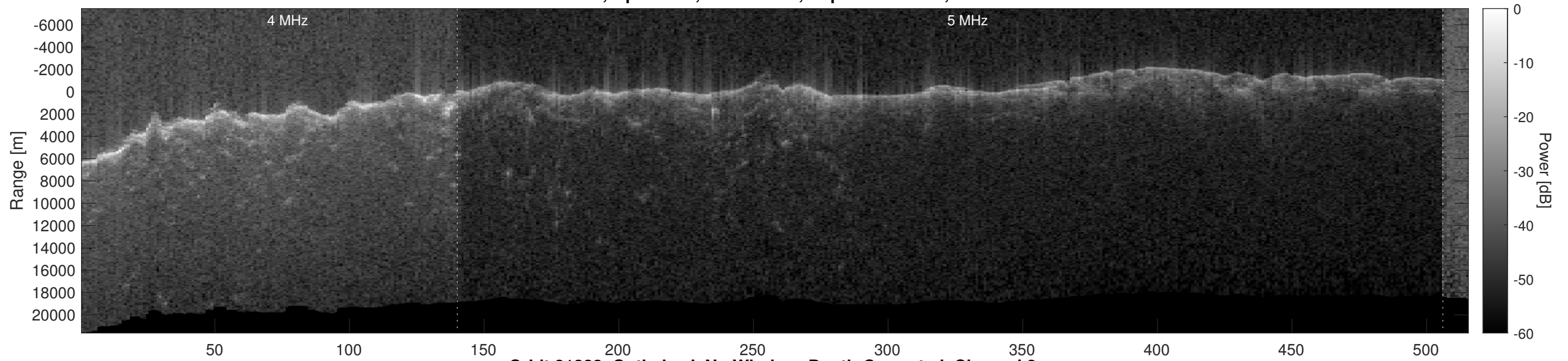
Orbit 21223, Optimized, No Window, Depth-Corrected, Channel 2
