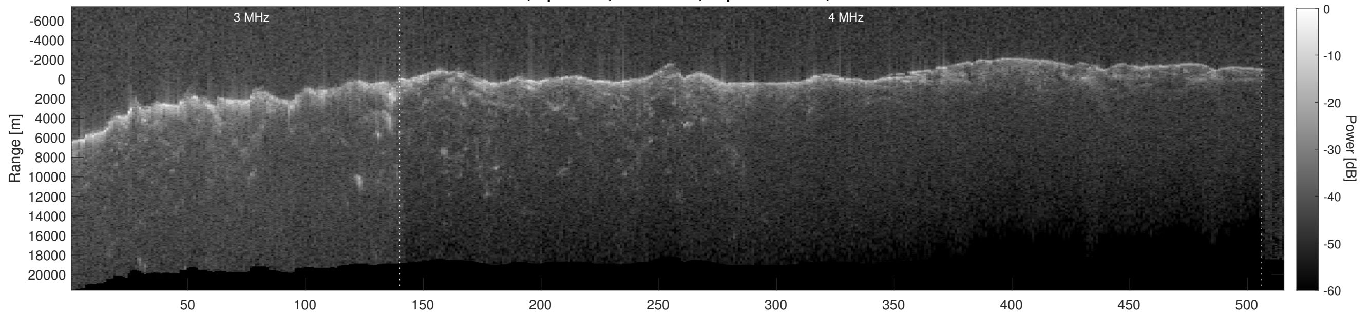
Orbit 21223, Depth-Corrected Cluttergram
