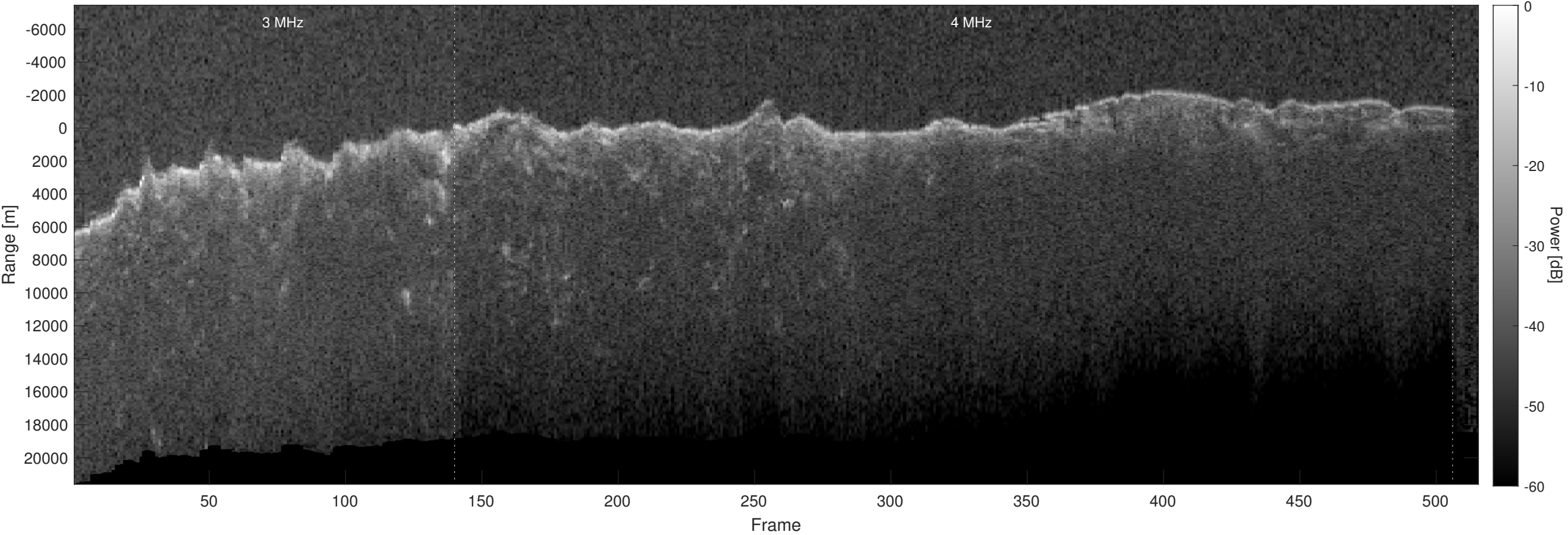
Orbit 21223, Optimized, Window, Depth-Corrected, Channel 2
