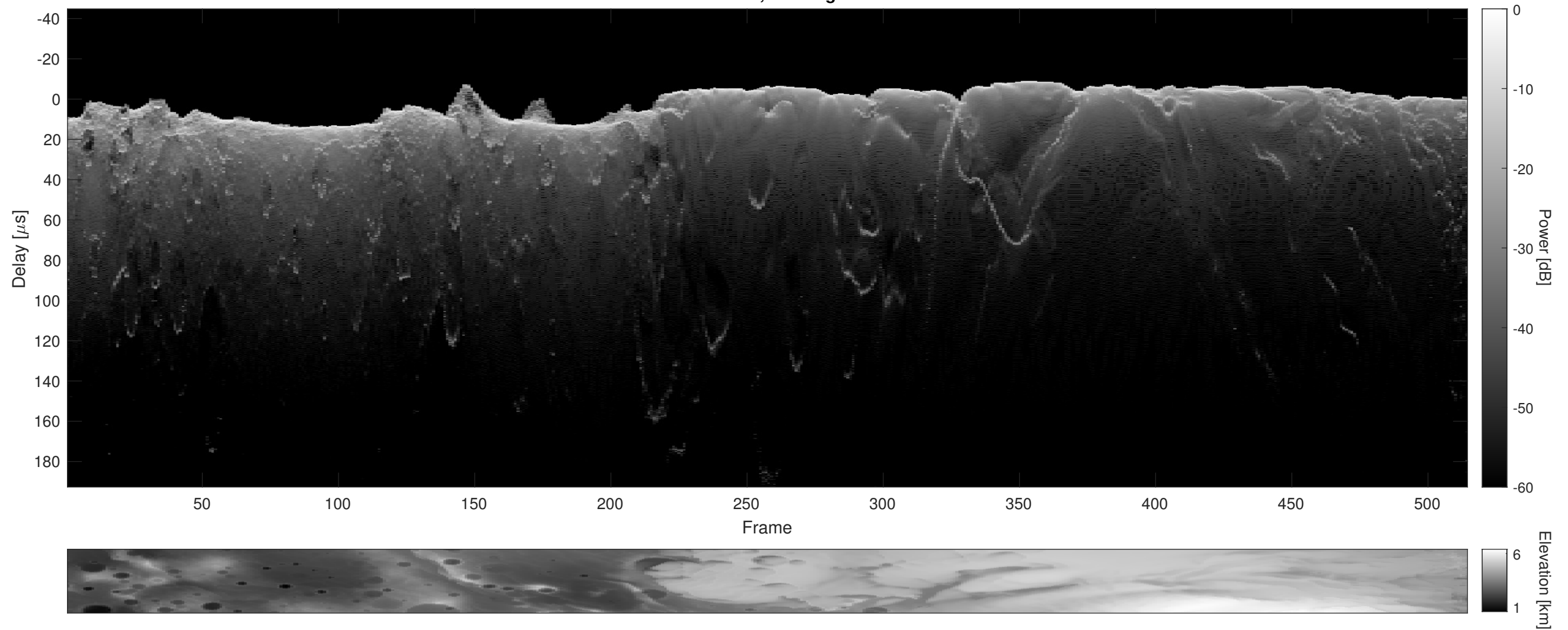
Orbit 21226, Cluttergram
