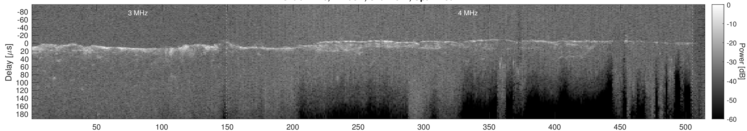
Orbit 21226, Cluttergram
