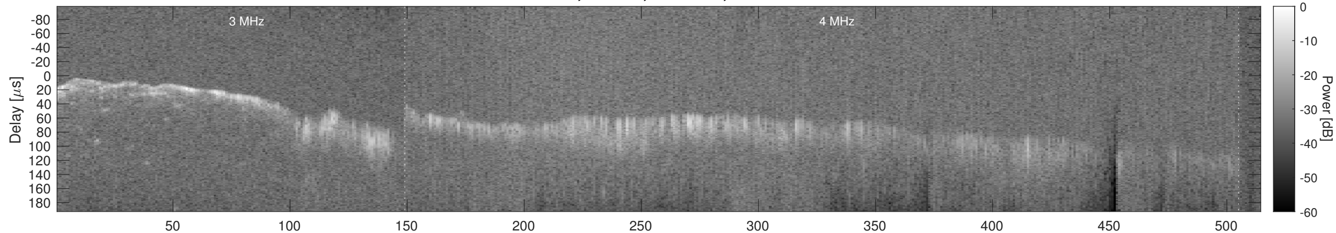
Orbit 21226, Window, Channel 2, Chapman
