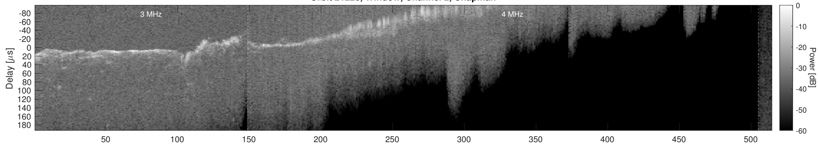
Orbit 21226, Window, Channel 2, Optimized
