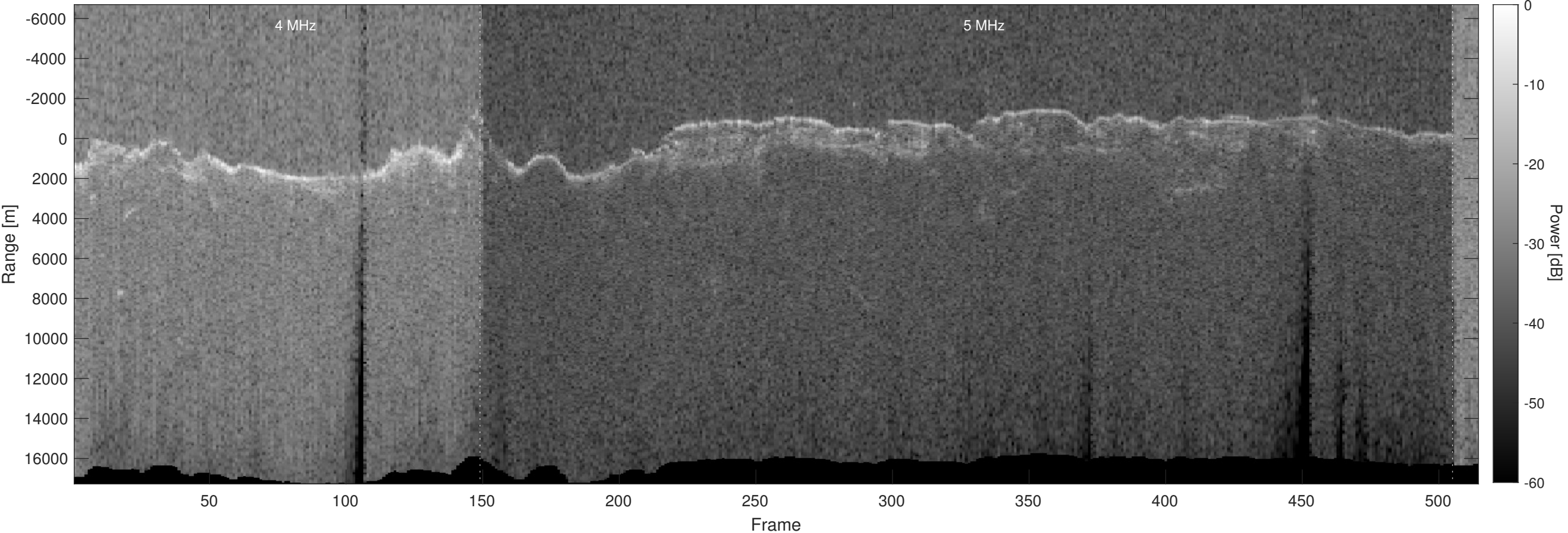
Orbit 21226, Optimized, Window, Depth-Corrected, Channel 2
