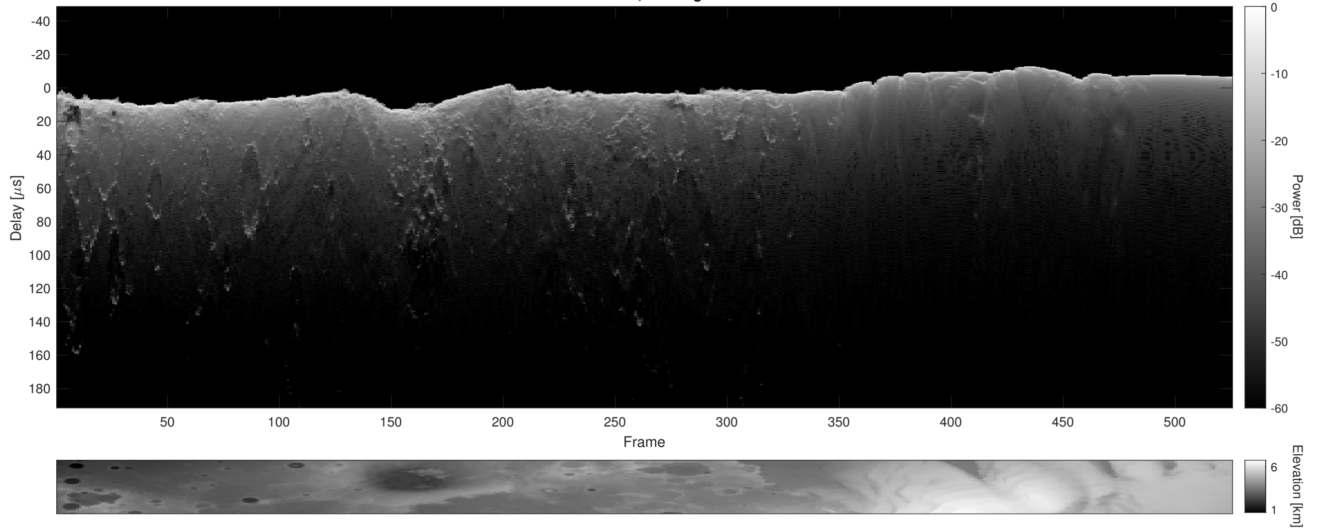
Orbit 21227, Cluttergram
