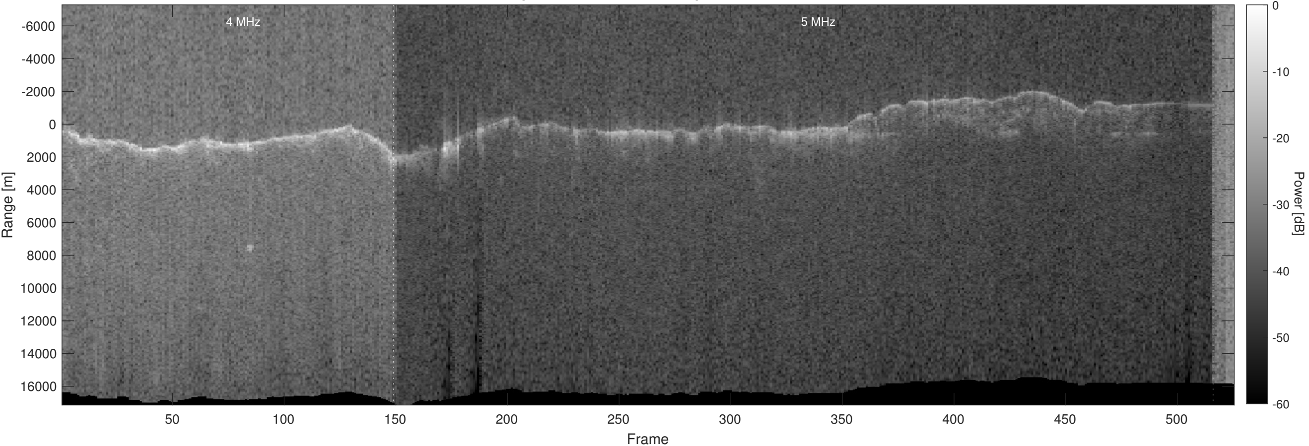
Orbit 21227, Optimized, No Window, Depth-Corrected, Channel 2
