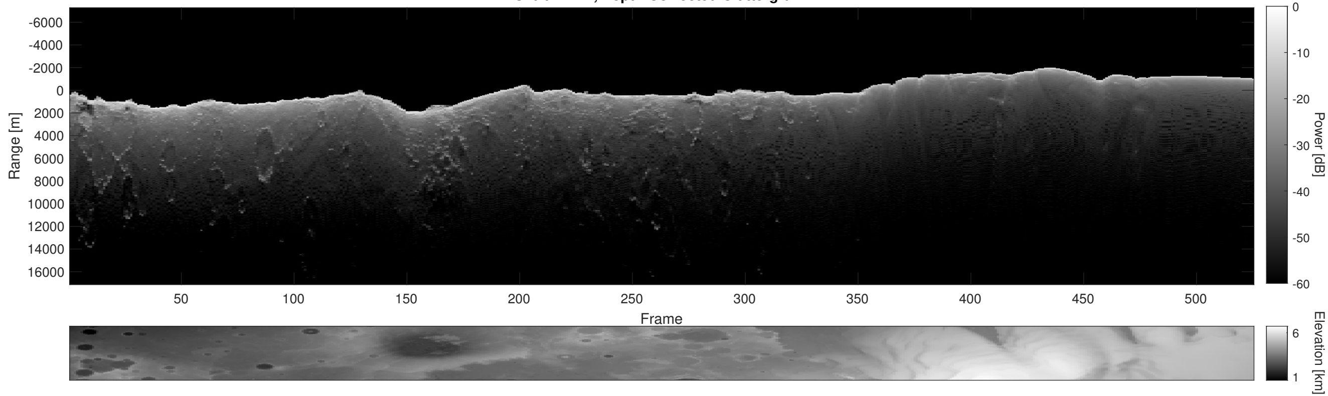
Orbit 21227, Depth-Corrected Cluttergram
