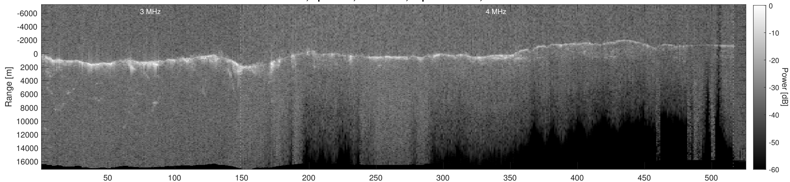
Orbit 21227, Depth-Corrected Cluttergram
