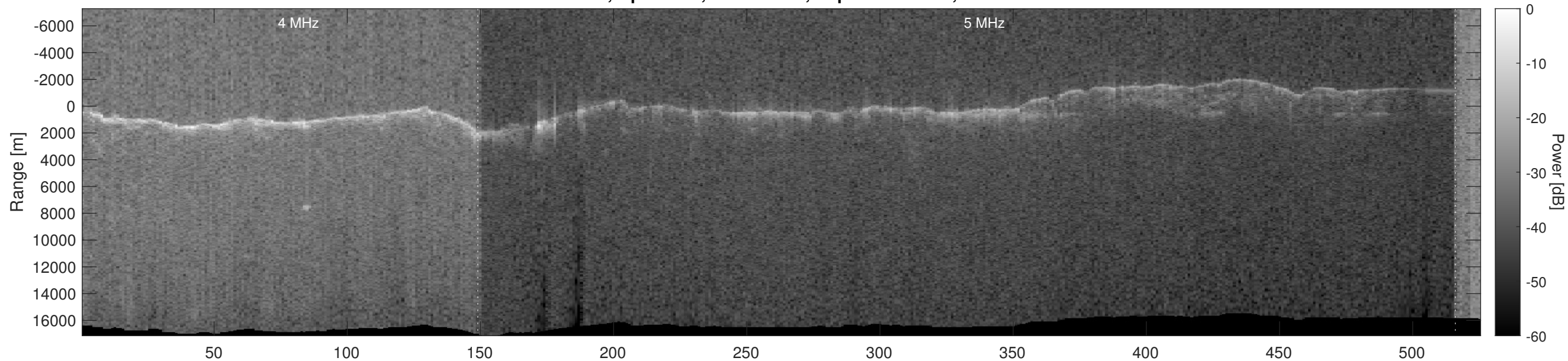
Orbit 21227, Optimized, No Window, Depth-Corrected, Channel 2
