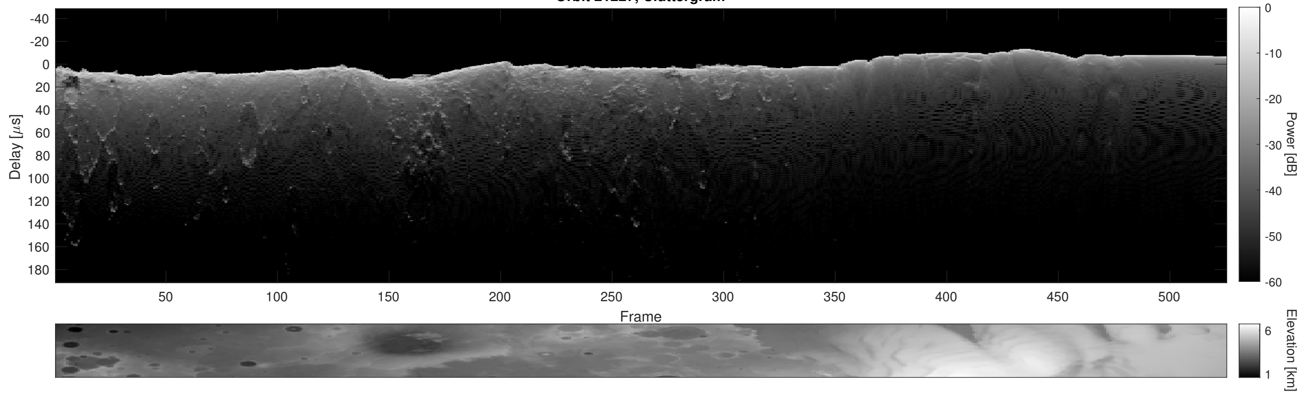
Orbit 21227, Cluttergram
