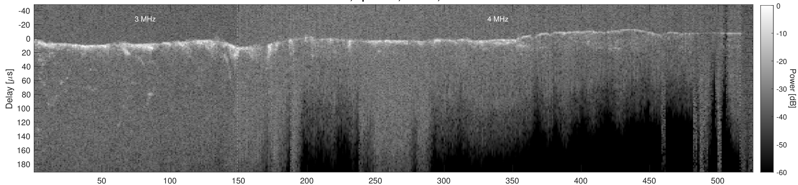
Orbit 21227, Cluttergram
