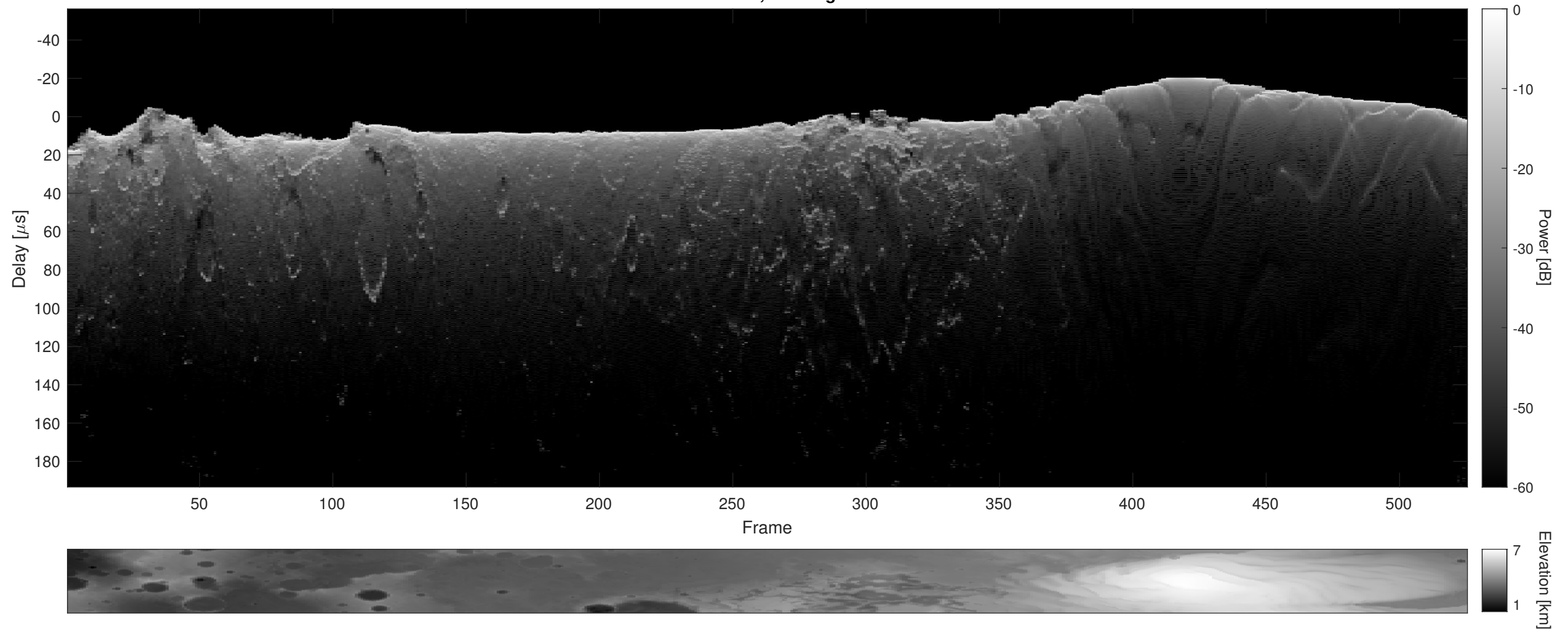
Orbit 21228, Cluttergram
