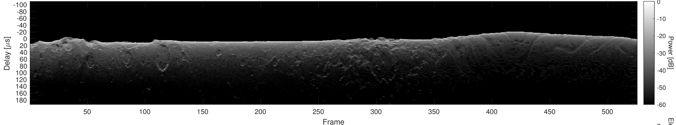
Orbit 21228, Cluttergram
