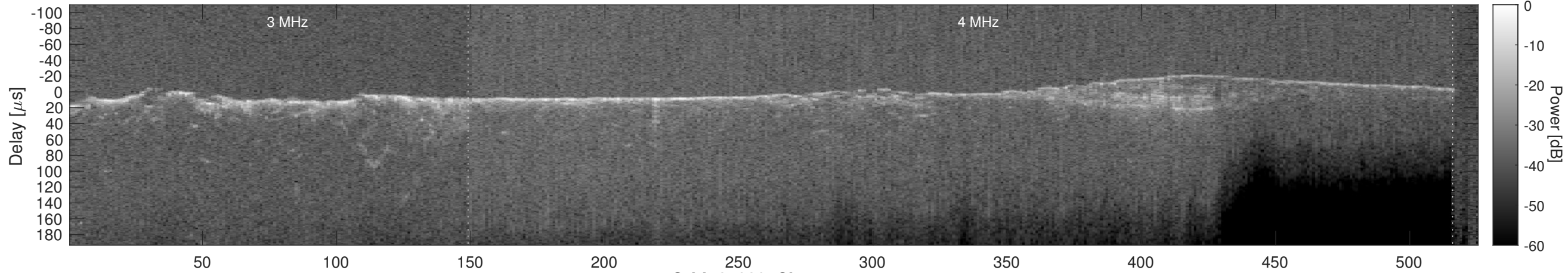
Orbit 21228, Cluttergram
