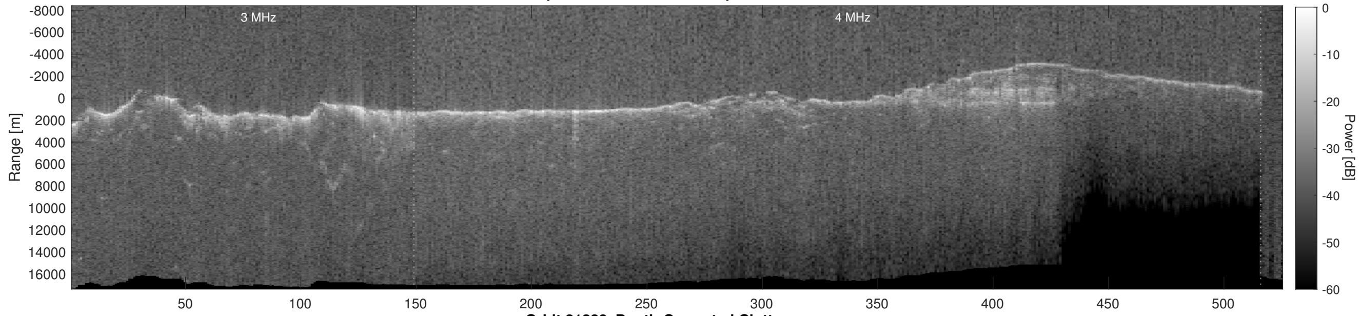
Orbit 21228, Depth-Corrected Cluttergram
