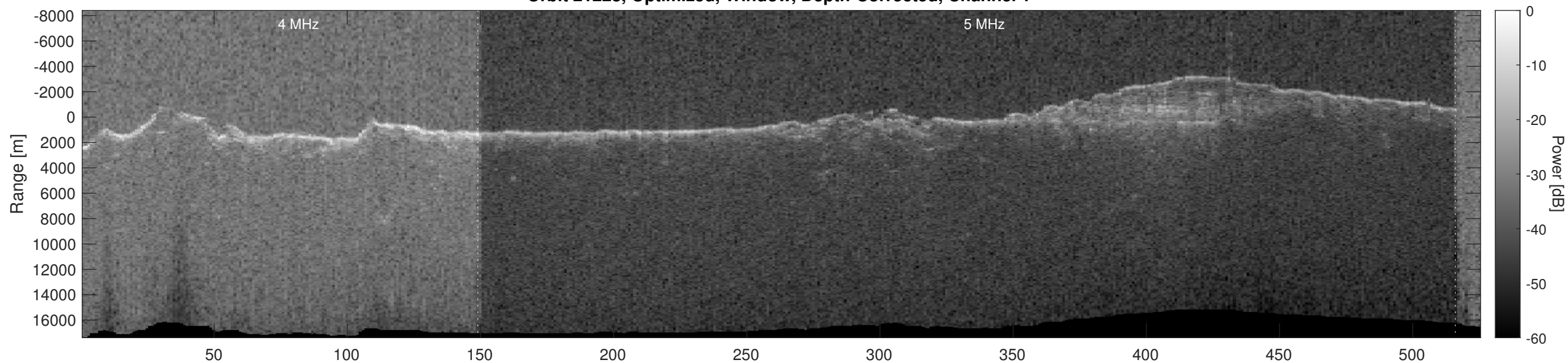
Orbit 21228, Optimized, Window, Depth-Corrected, Channel 2
