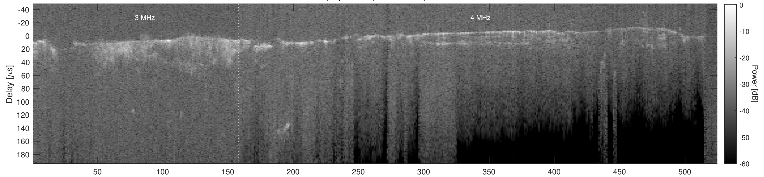
Orbit 21229, Cluttergram
