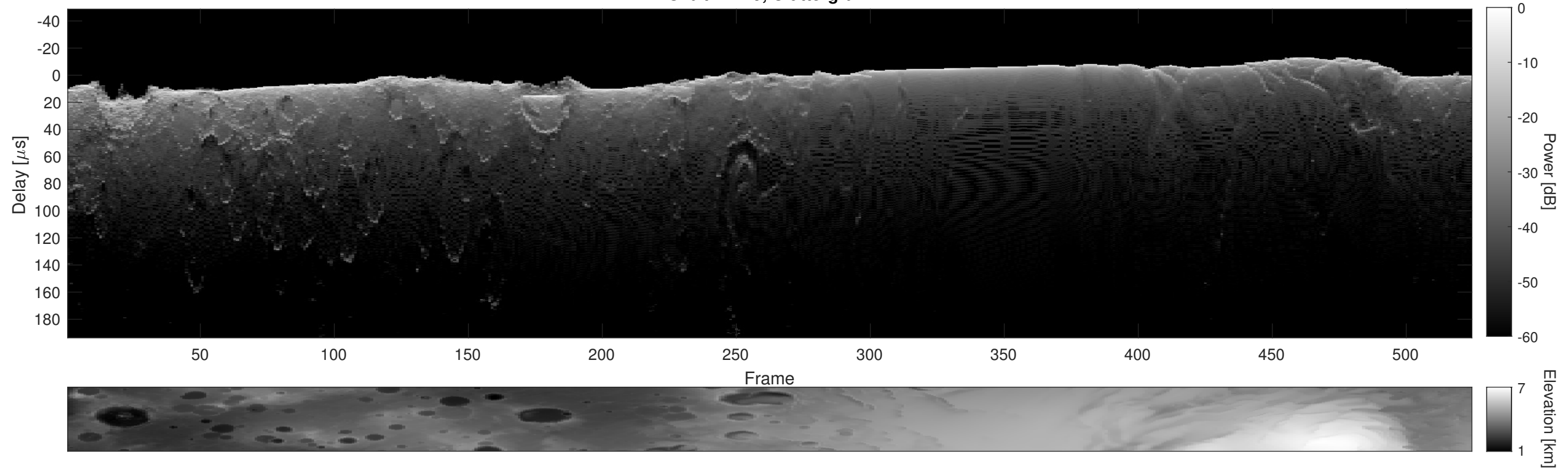
Orbit 21229, Cluttergram
