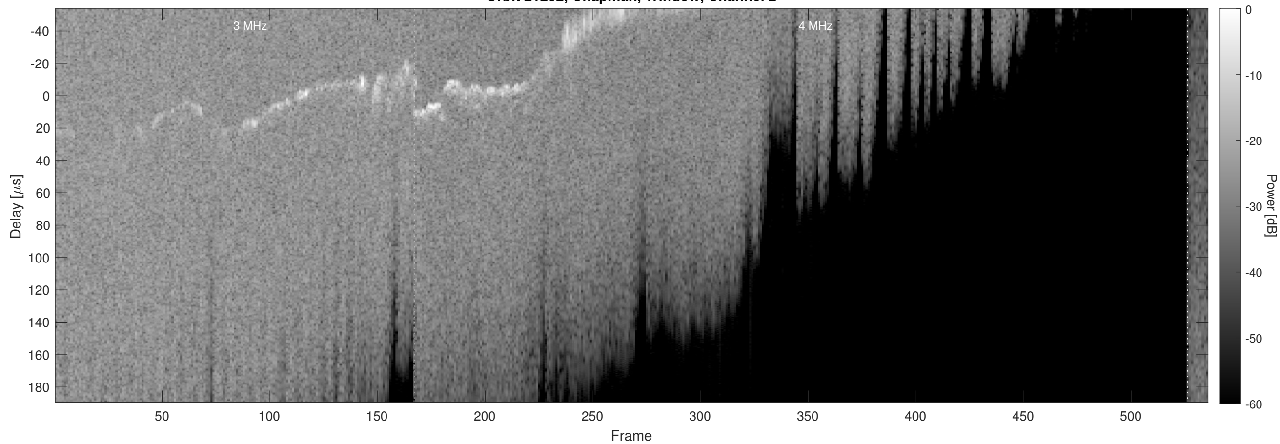
Orbit 21232, Chapman, Window, Channel 2
