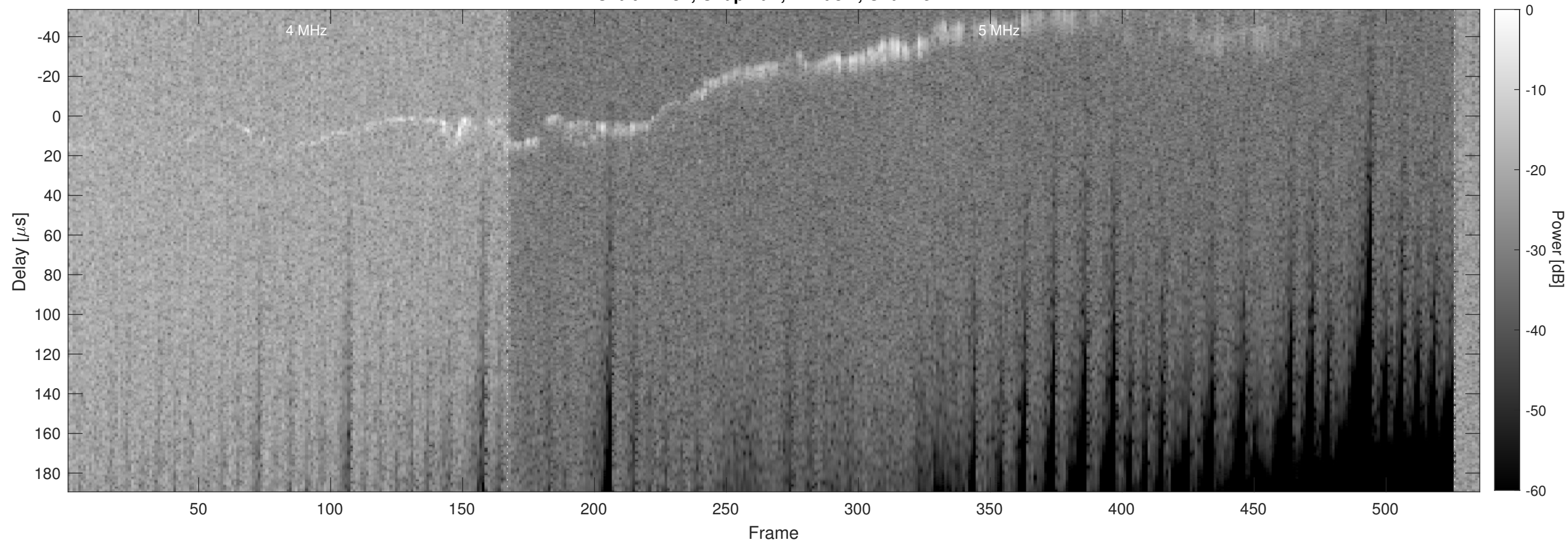
Orbit 21232, Chapman, Window, Channel 2
