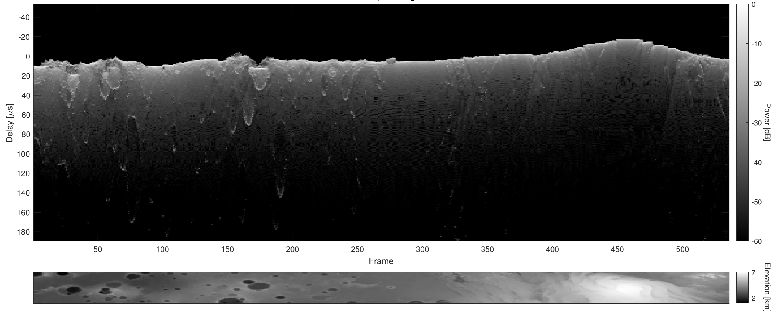
Orbit 21232, Cluttergram
