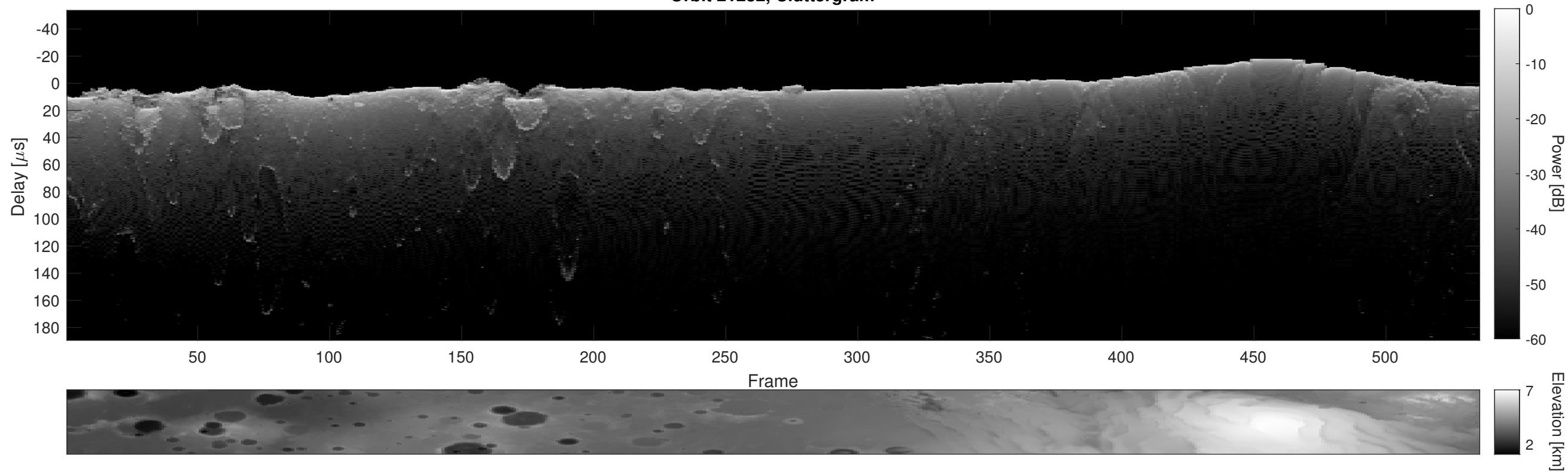
Orbit 21232, Cluttergram
