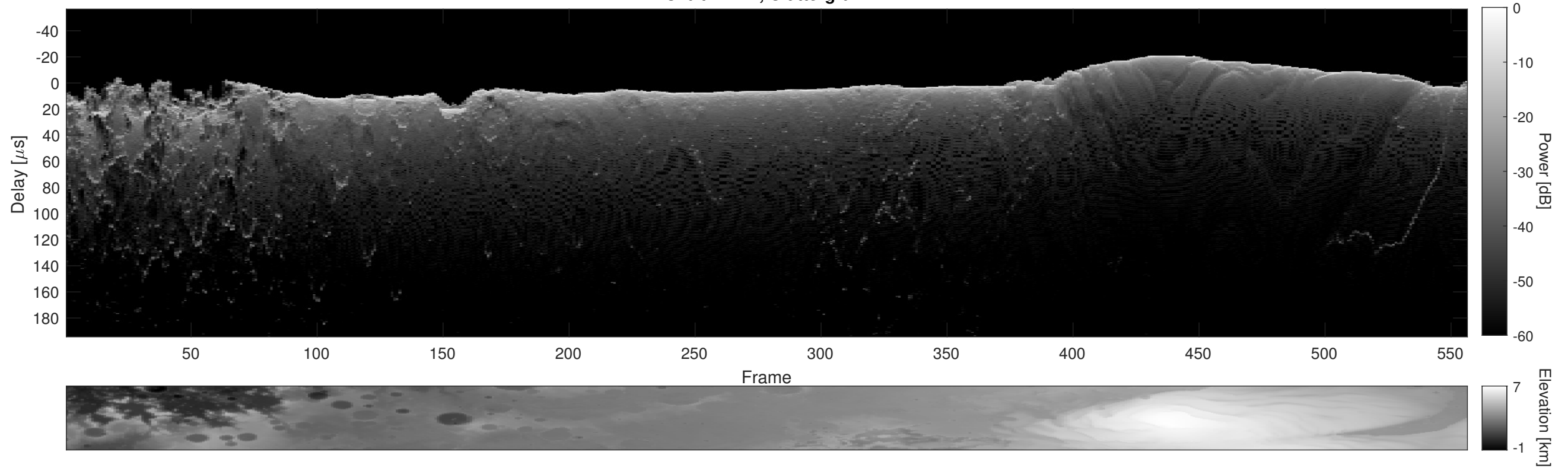
Orbit 21242, Cluttergram
