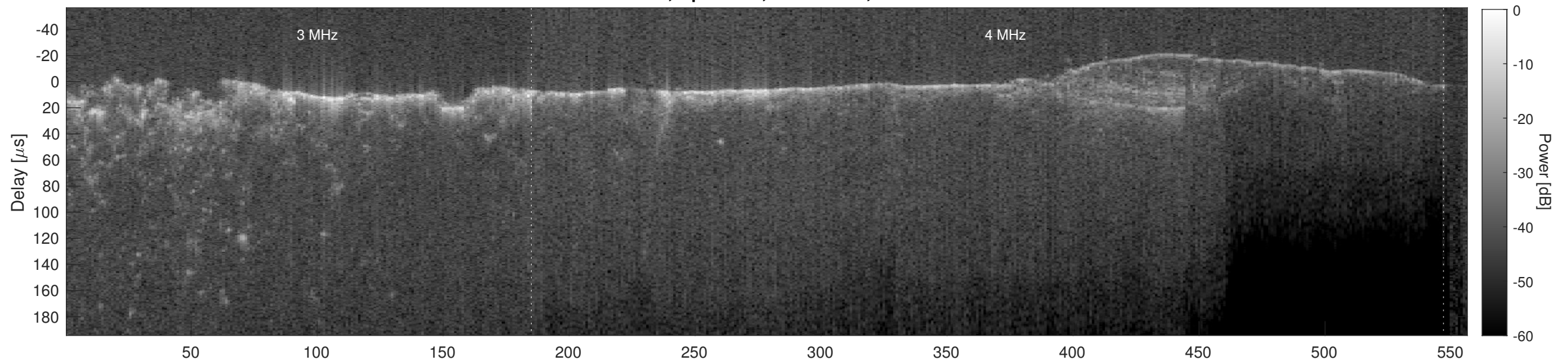
Orbit 21242, Cluttergram
