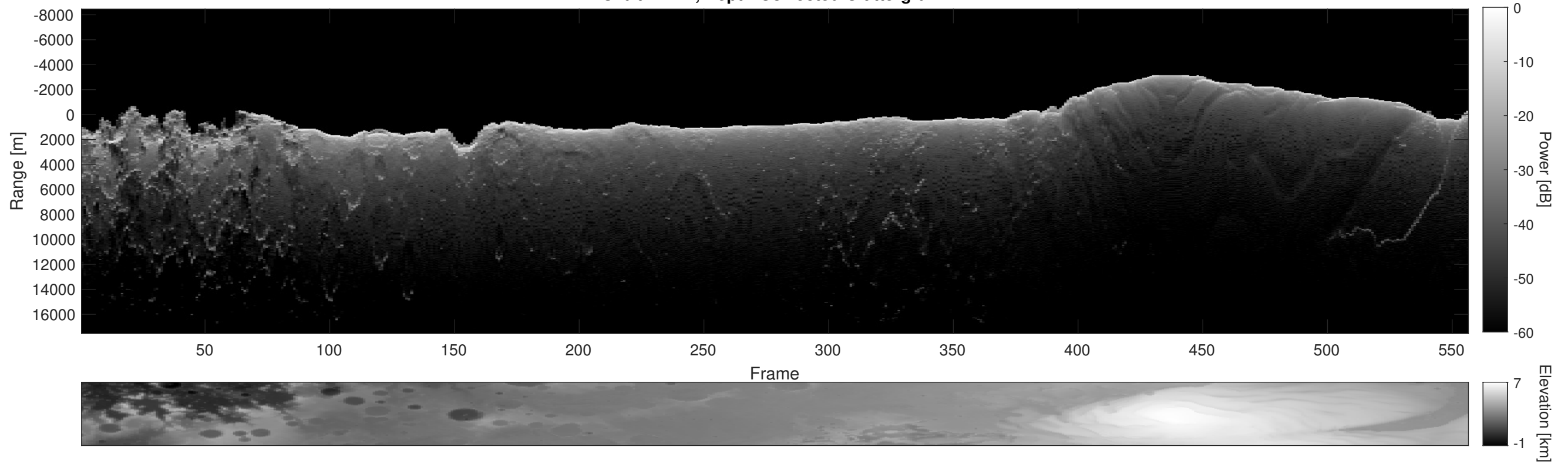
Orbit 21242, Depth-Corrected Cluttergram
