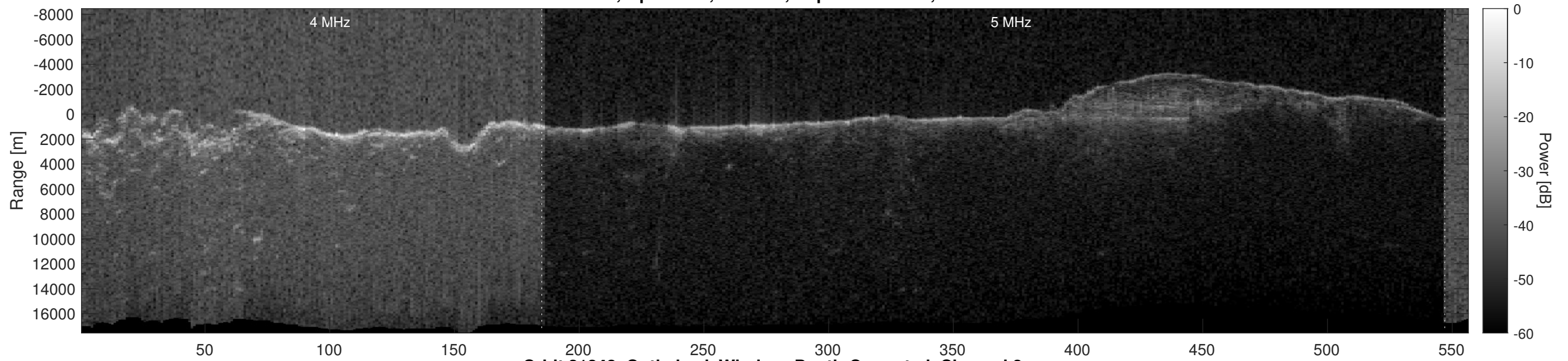
Orbit 21242, Optimized, Window, Depth-Corrected, Channel 2
