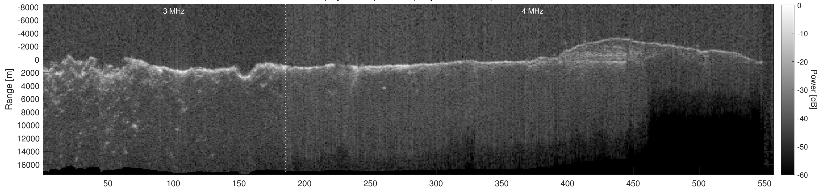
Orbit 21242, Depth-Corrected Cluttergram
