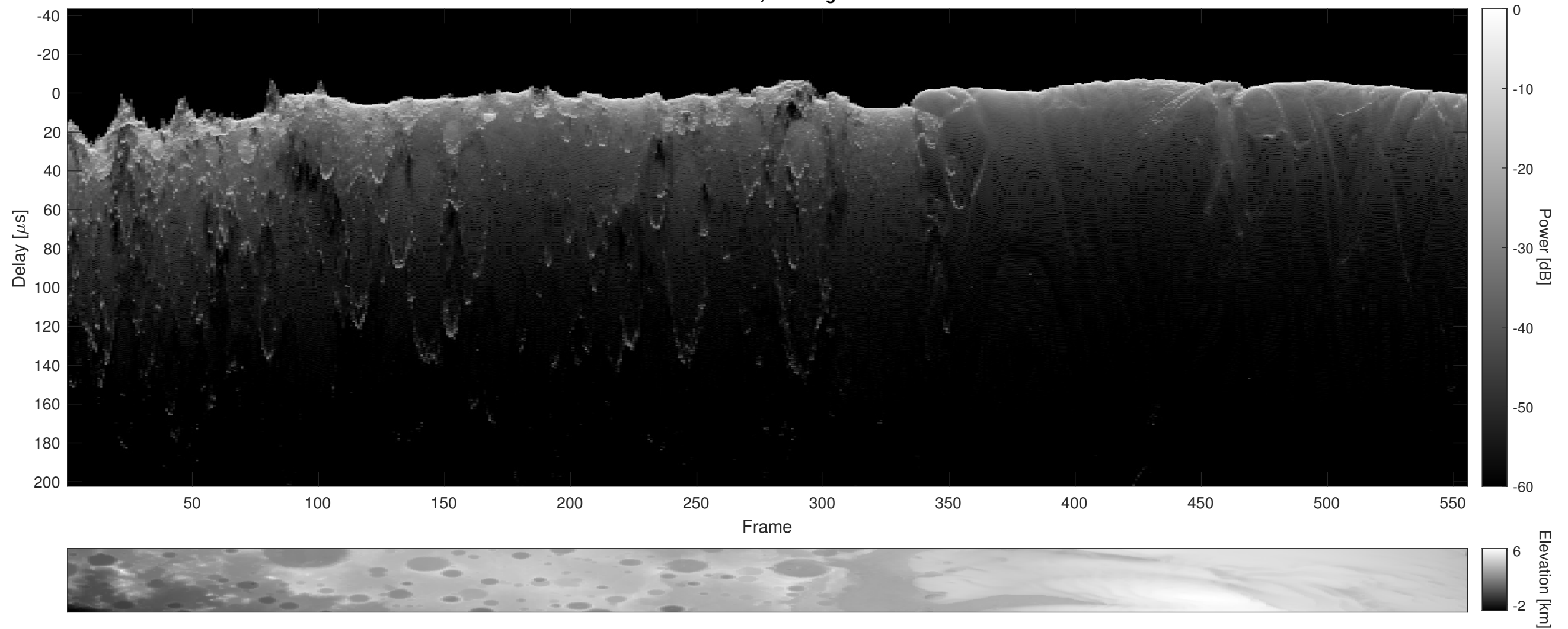
Orbit 21244, Cluttergram
