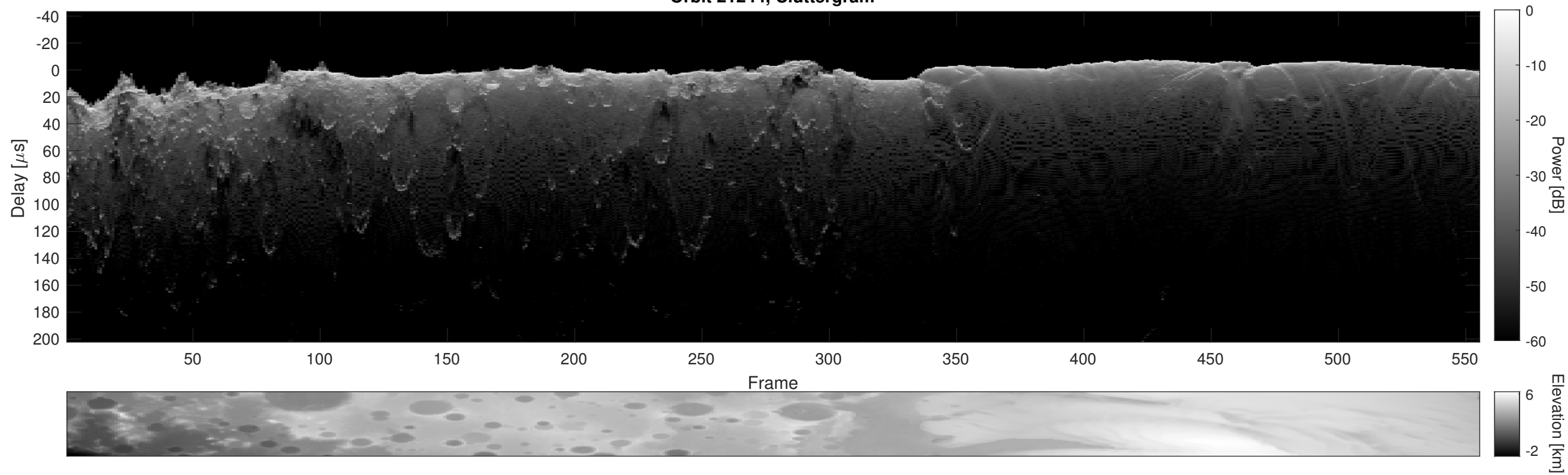
Orbit 21244, Cluttergram
