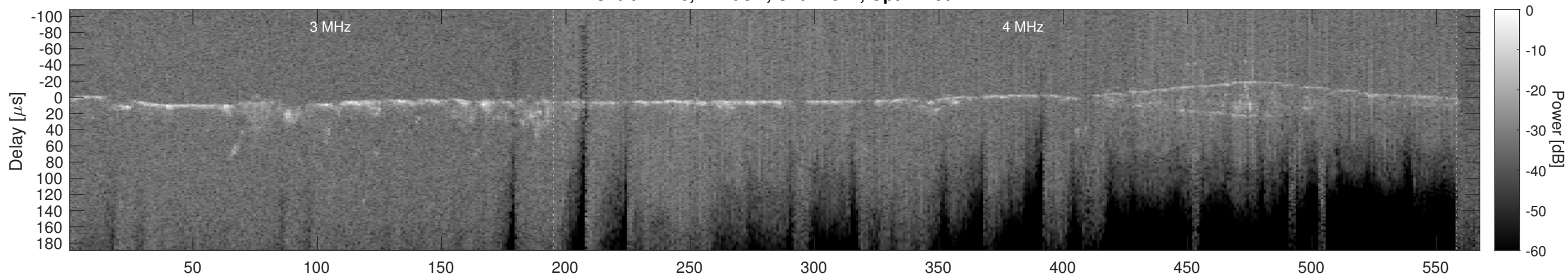
Orbit 21246, Cluttergram
