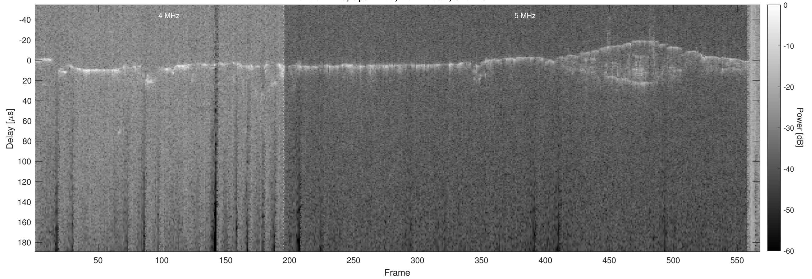
Orbit 21246, Optimized, No Window, Channel 2
