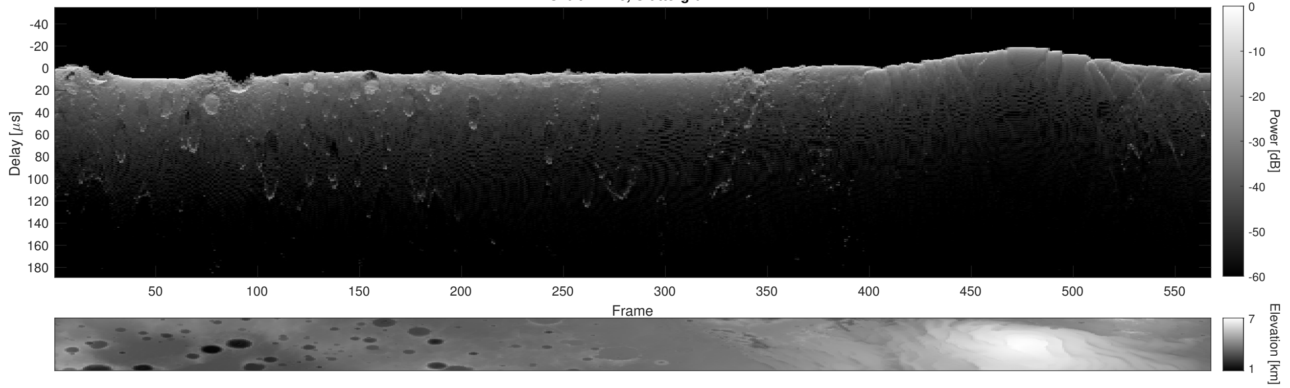
Orbit 21246, Cluttergram
