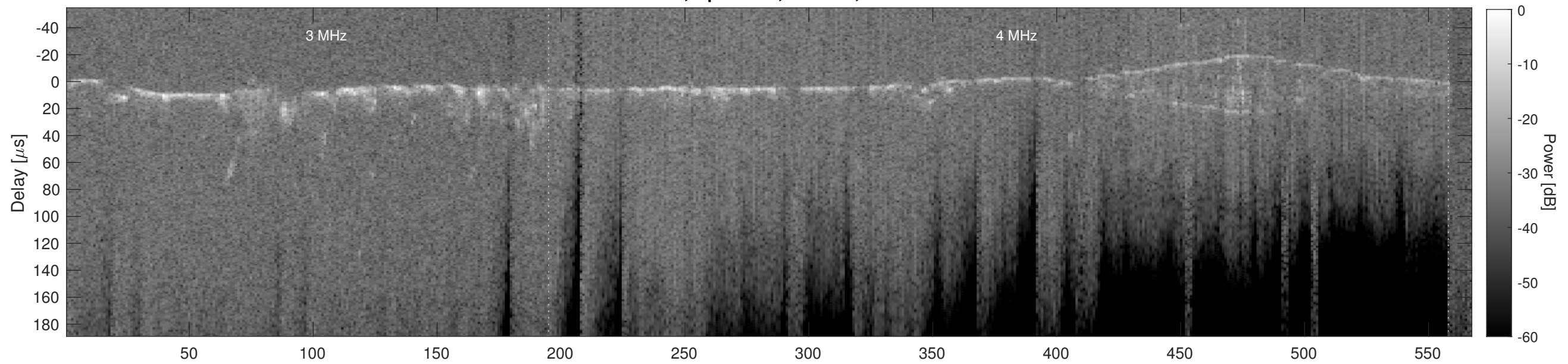
Orbit 21246, Cluttergram
