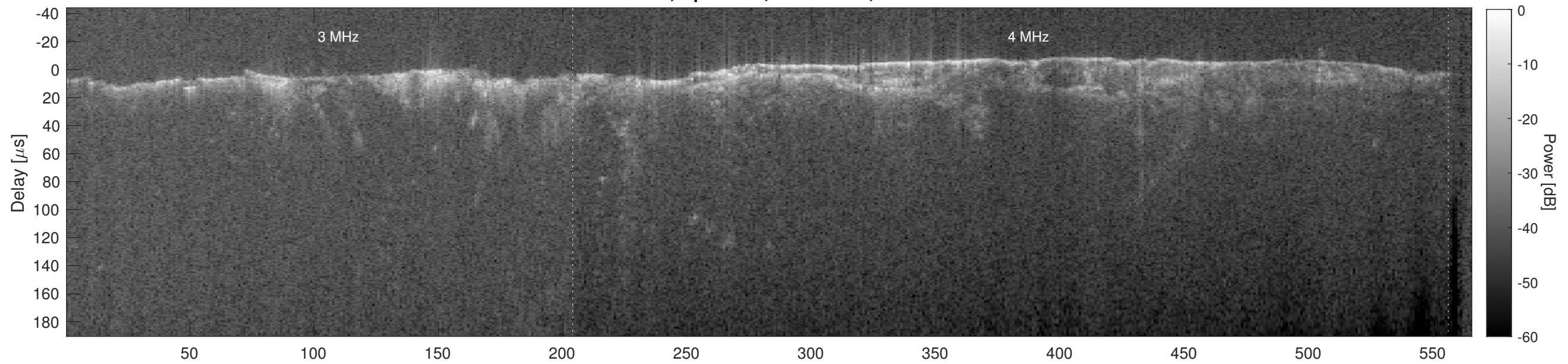
Orbit 21247, Cluttergram
