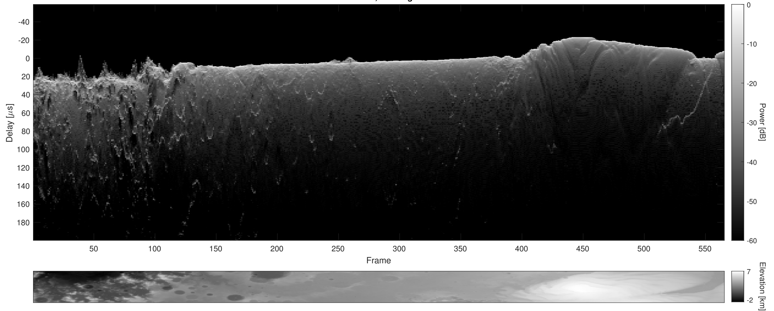
Orbit 21249, Cluttergram
