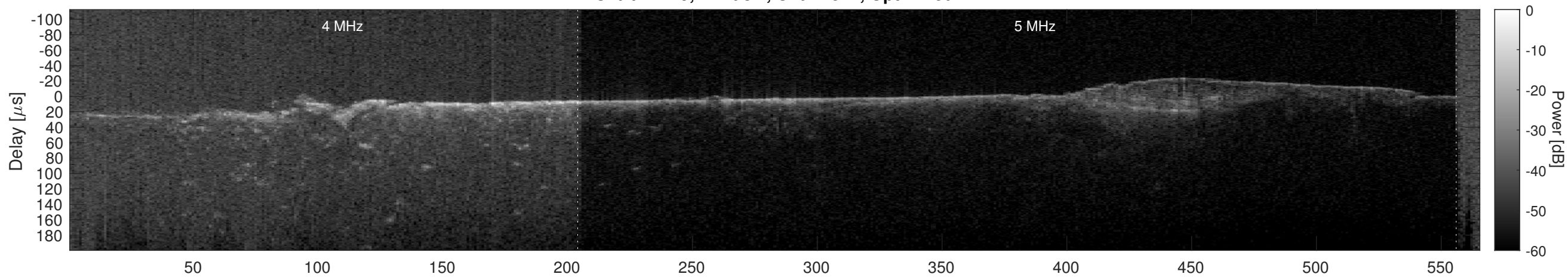
Orbit 21249, Cluttergram
