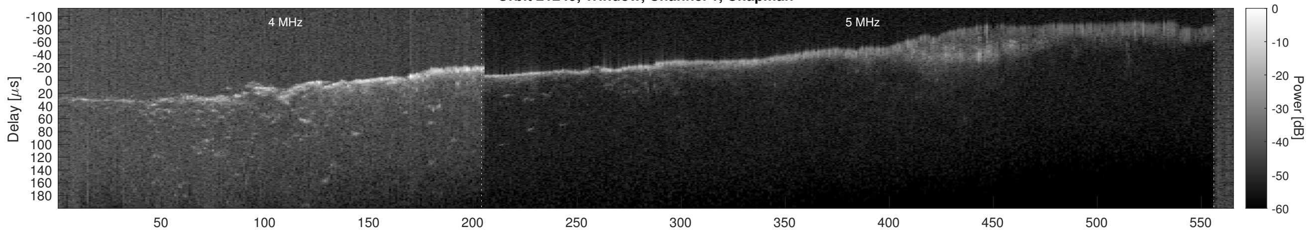
Orbit 21249, Window, Channel 1, Optimized
