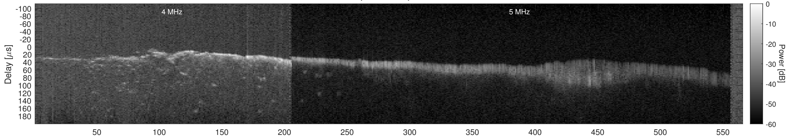
Orbit 21249, Window, Channel 1, Chapman
