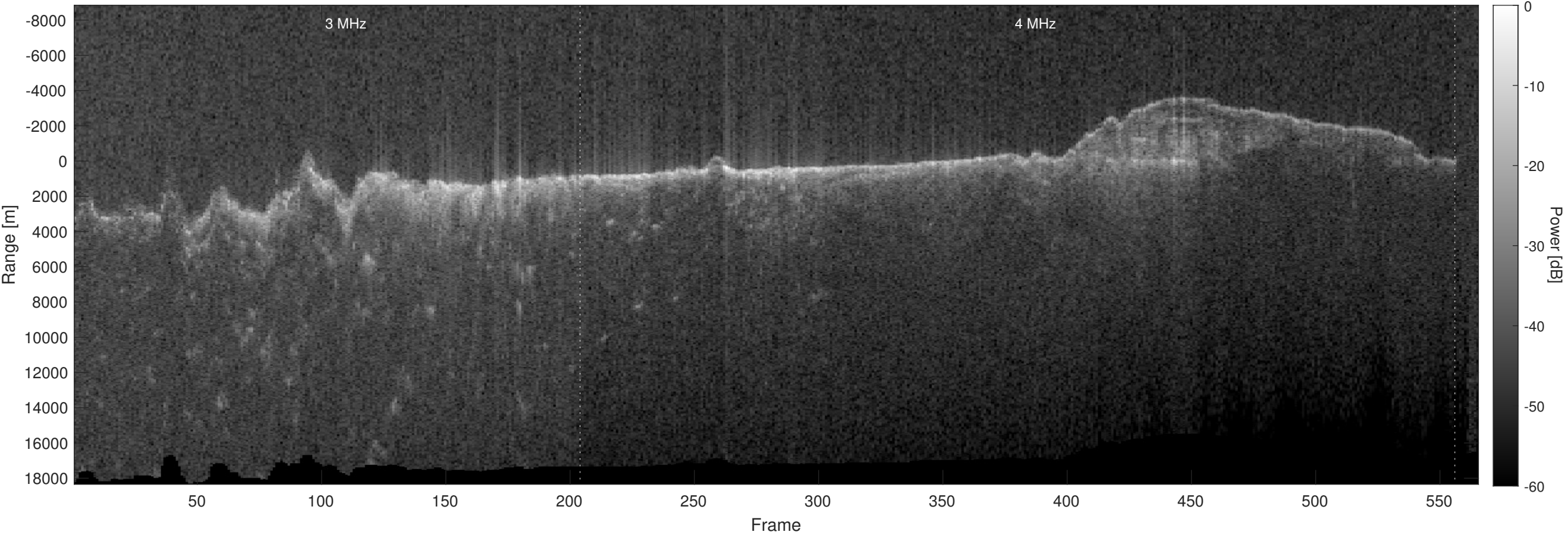
Orbit 21249, Optimized, No Window, Depth-Corrected, Channel 2
