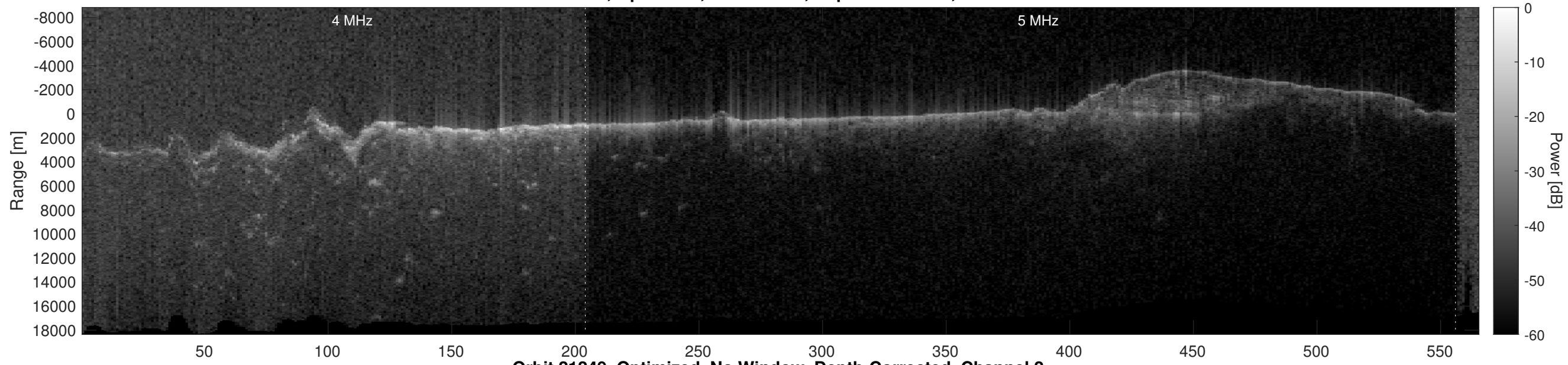
Orbit 21249, Optimized, No Window, Depth-Corrected, Channel 2
