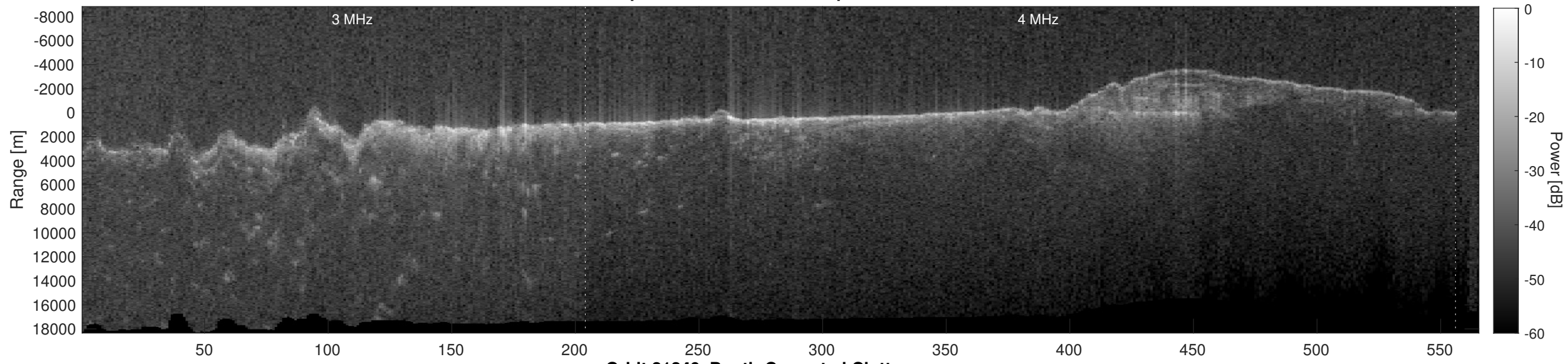
Orbit 21249, Depth-Corrected Cluttergram
