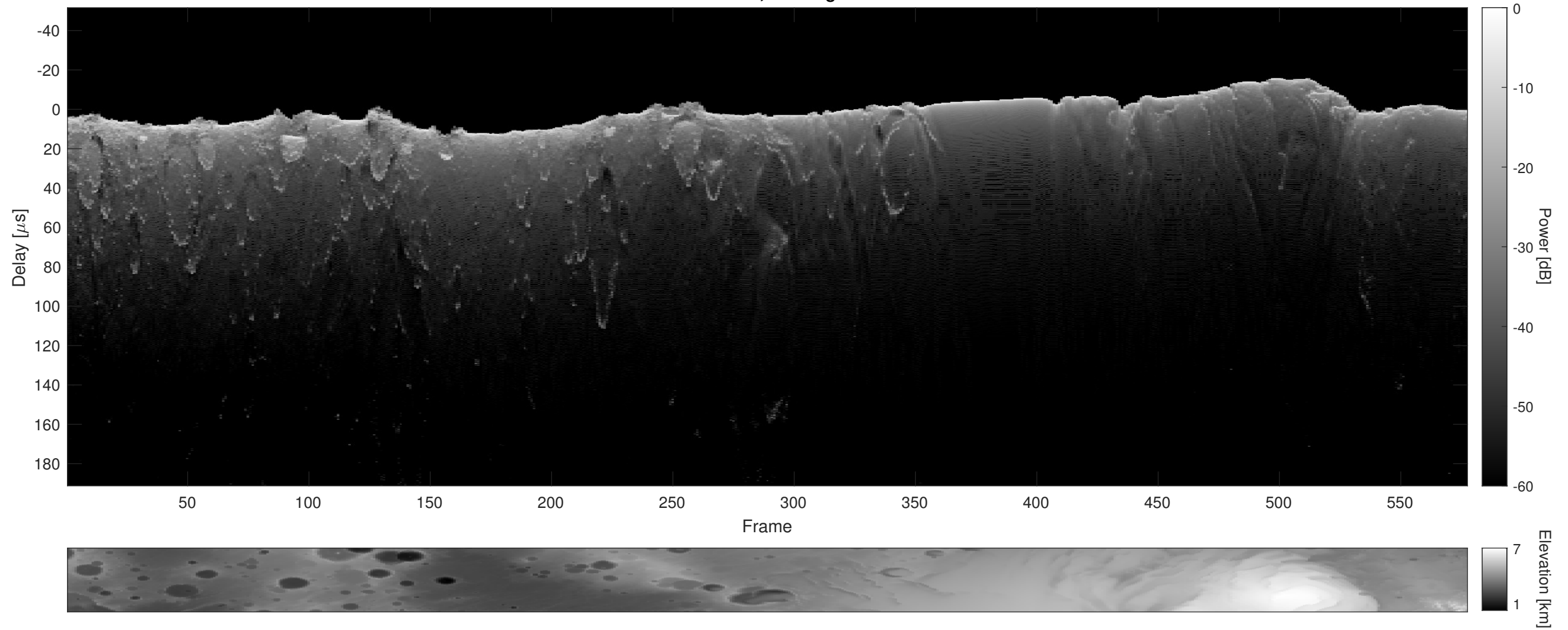
Orbit 21250, Cluttergram
