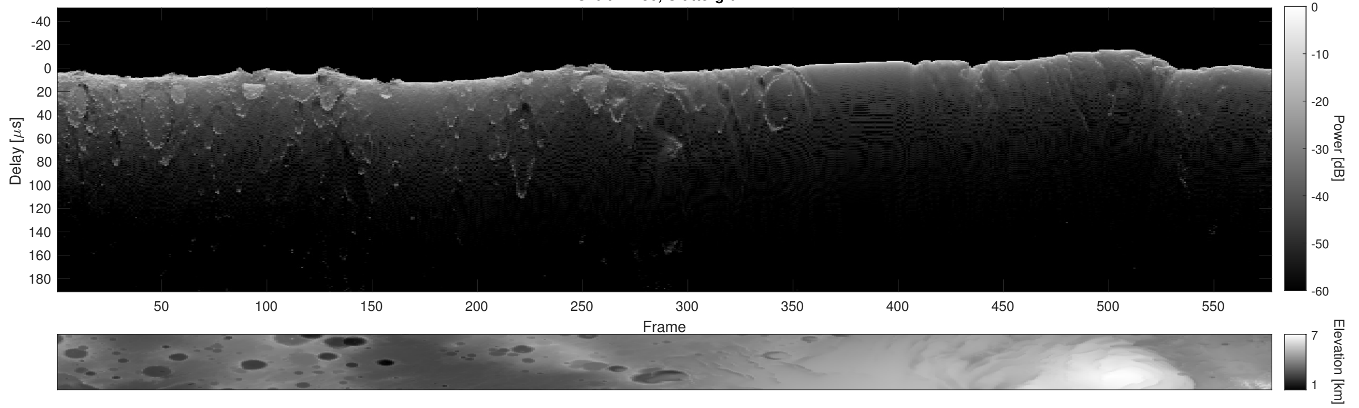
Orbit 21250, Cluttergram
