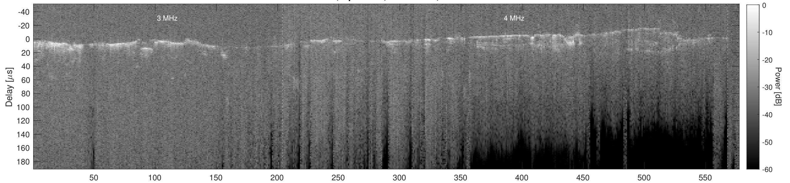
Orbit 21250, Cluttergram
