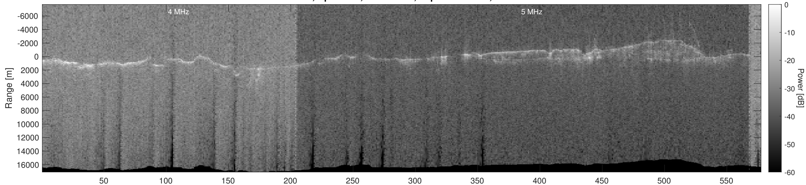
Orbit 21250, Optimized, No Window, Depth-Corrected, Channel 2
