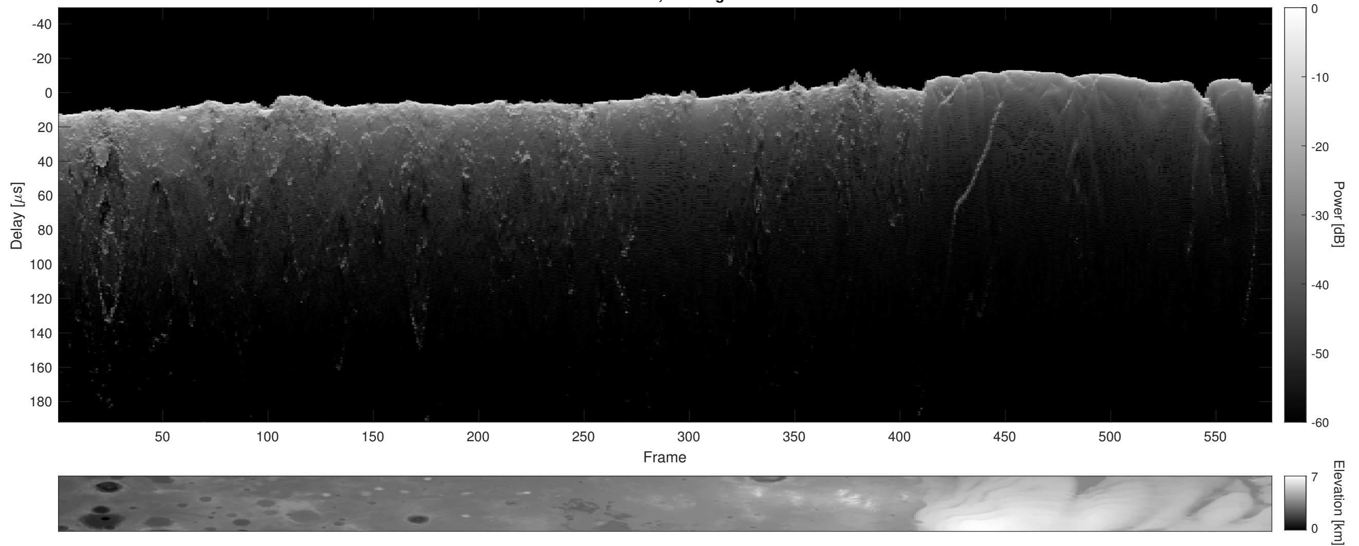
Orbit 21252, Cluttergram
