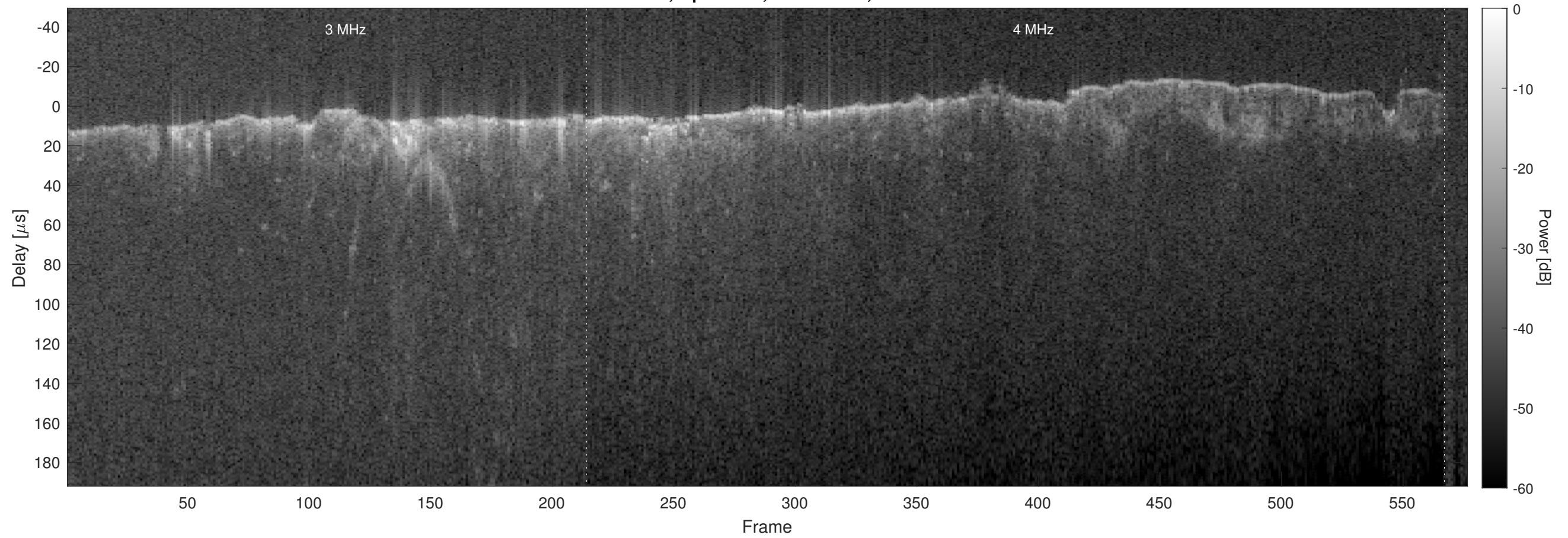
Orbit 21252, Optimized, No Window, Channel 2
