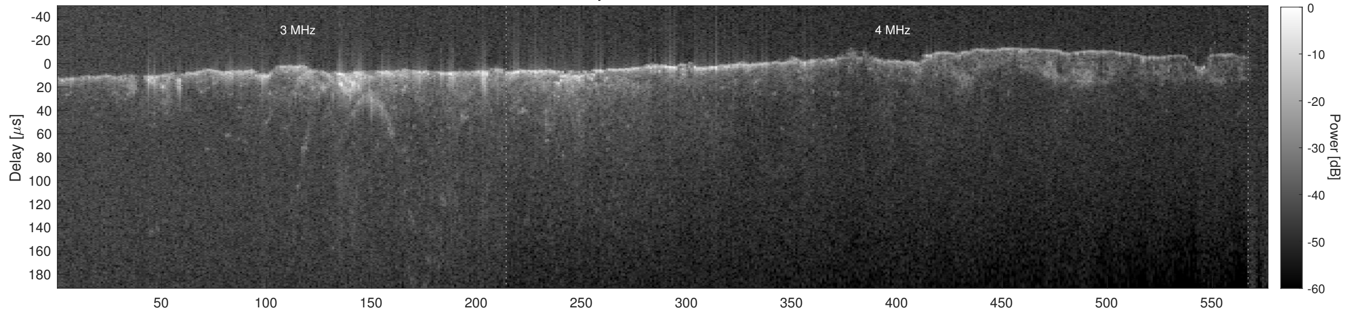
Orbit 21252, Cluttergram
